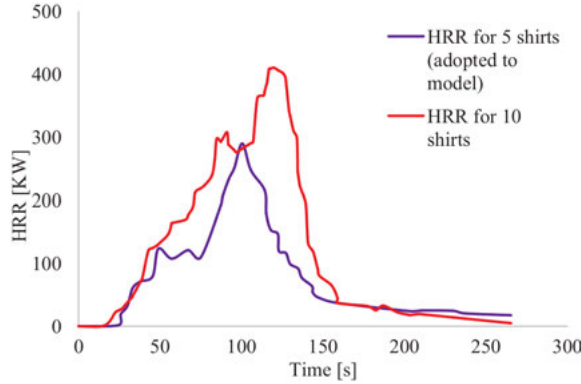
Fig. 7. Heat release rate for curtain [27]
