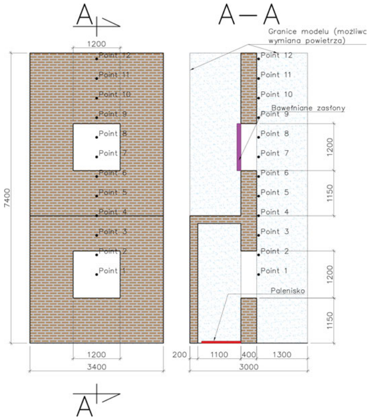
Fig. 5. Scheme and dimensions adopted for exemplary model
