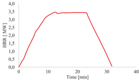
Fig. 6. Heat release rate adopted for numerical model in accordance with BS8414-1 [10]
