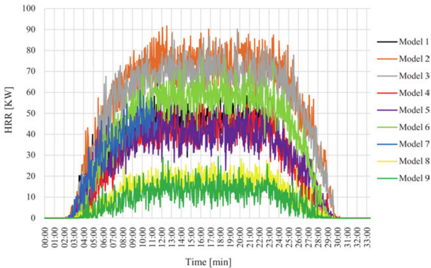
Fig. 19. HRR on the surface of the window opening from which the fire escapes
