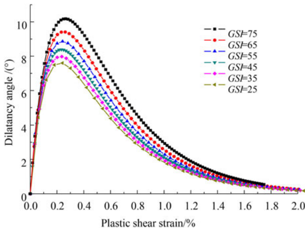
Fig. 6. Improved nonlinear dilatancy angle model of sandstone
