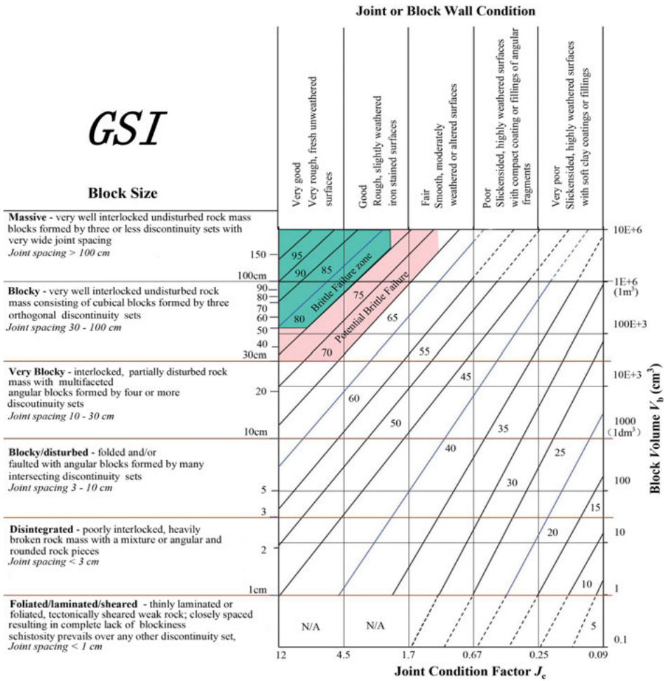
Fig. 1. Schematic diagram of quantifying GSI surrounding rock rating system
