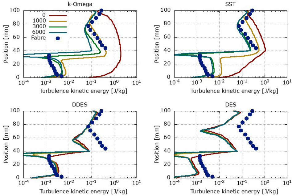
Figure 5: Profiles of the turbulent kinetic energy, k , in the centre plane at x_3 = 9 m (see Fig. 1) for four different turbulence models (top left – standard k-\omega model, top right – k\omega SST model, bottom left – hybrid SST–DDES model, bottom right – hybrid SST–DES model) and four different damping factors ( B = 0, 1000, 3000, \text{ and } 6000 ) in comparison with experimental data from Fabre et al. [2].
