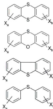
Fig. 1. Structures of polychlorinated thianthrenes, phenoxatynes, dibenzothiophenes and diphenyl thioethers.
