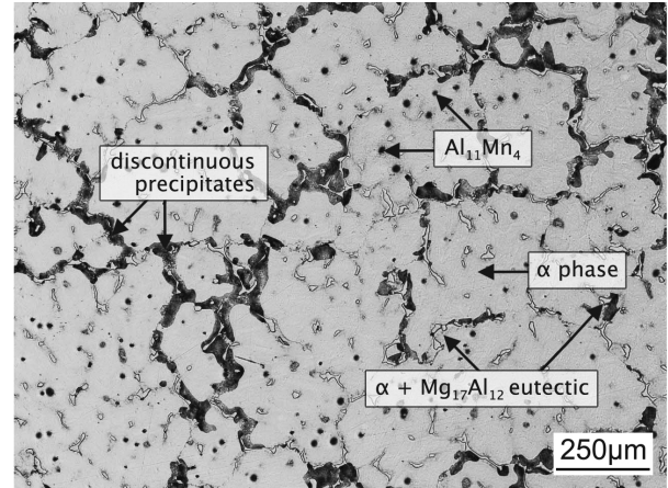
Fig. 2. OM microstructure of the as-cast AZ91 alloy
