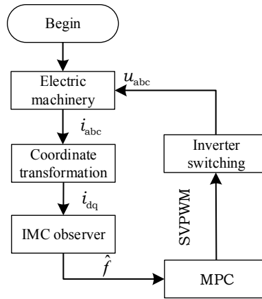
Fig. 4. Block diagram of model mismatch strategy based on internal model control observer
