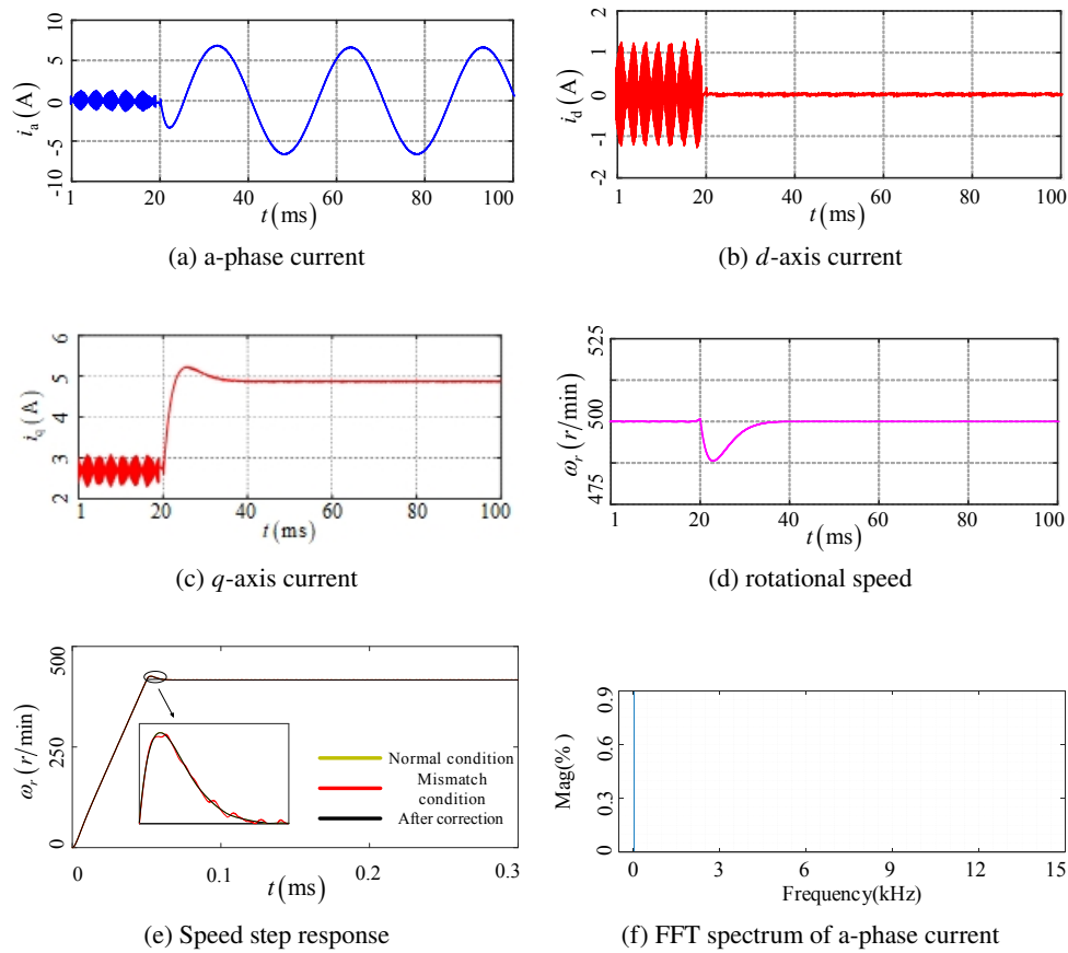
Fig. 11. Experimental waveform of three vector model predictive current control based on self-correcting under the condition of motor parameter mismatch
