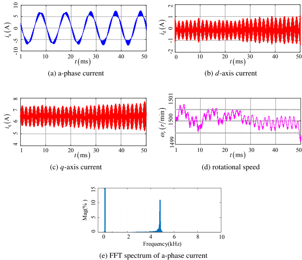
Fig. 7. Experimental waveform of three vector model predictive current control under the condition of motor parameter mismatch
