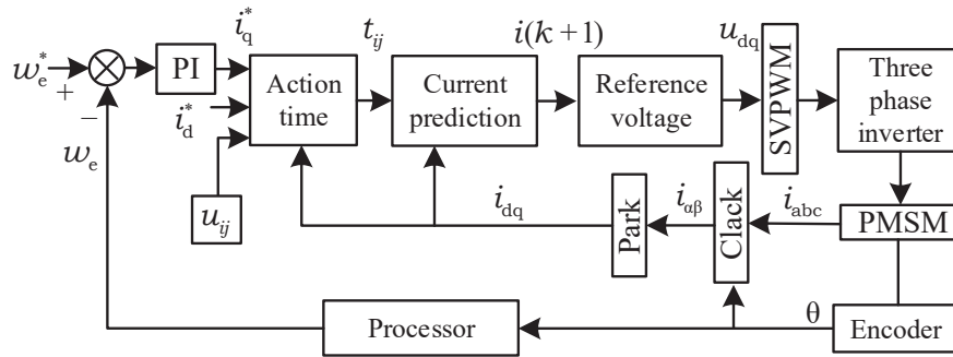
Fig. 1. Block diagram of the three-vector-based model predictive current control system
