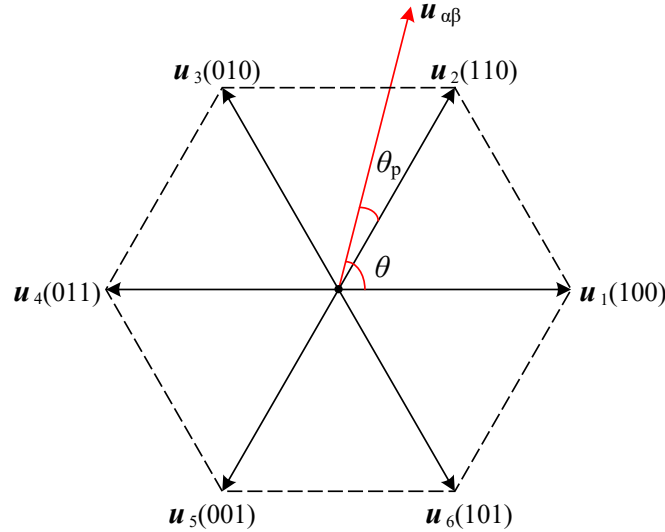
Fig. 2. Schematic diagram of reference voltage vector position angle
