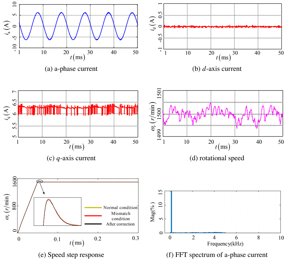
Fig. 8. Experimental waveform of three vector model predictive current control based on self-correcting under the condition of motor parameter mismatch
