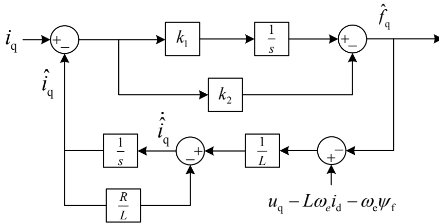
(b) IMC observer of q -axis current
