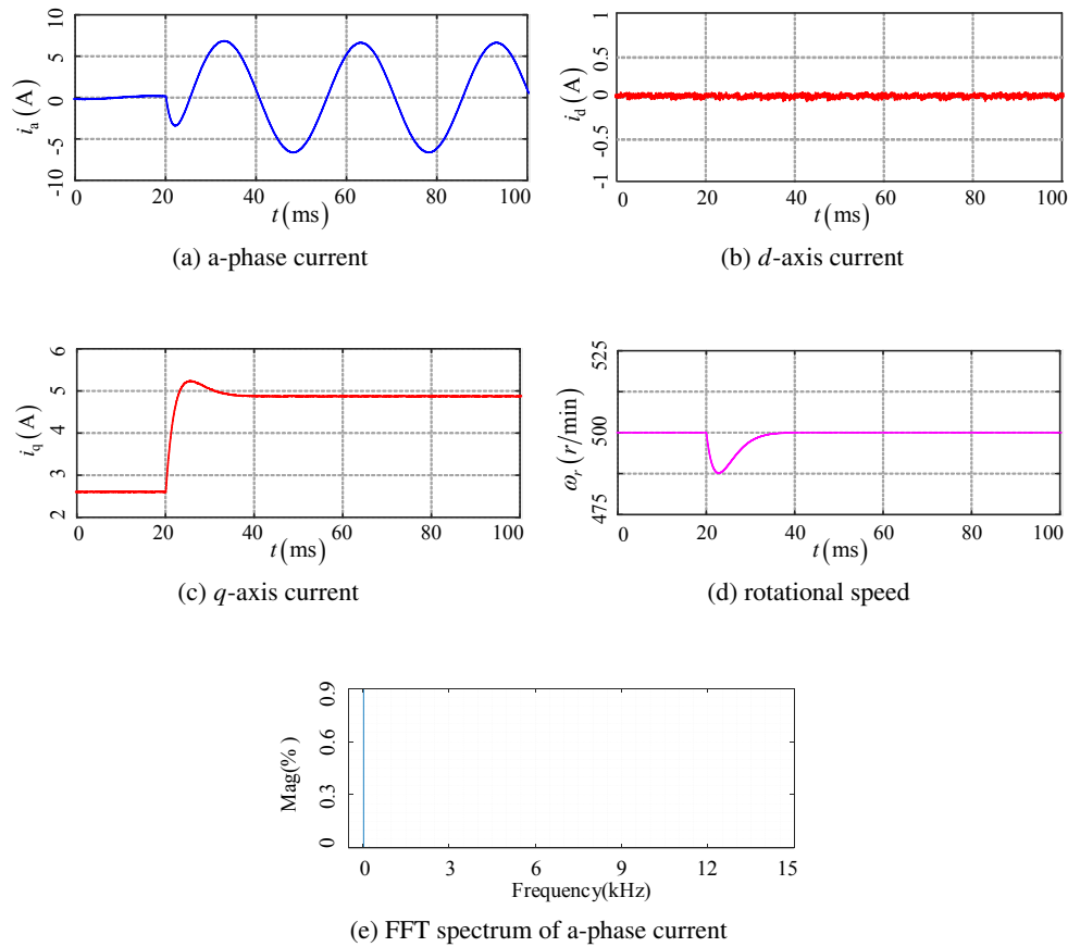
Fig. 9. Waveform of three vector model predictive current control under rated motor parameters
