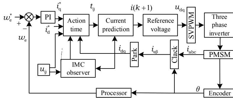
Fig. 5. Block diagram of model predictive current control based on internal model control observer
