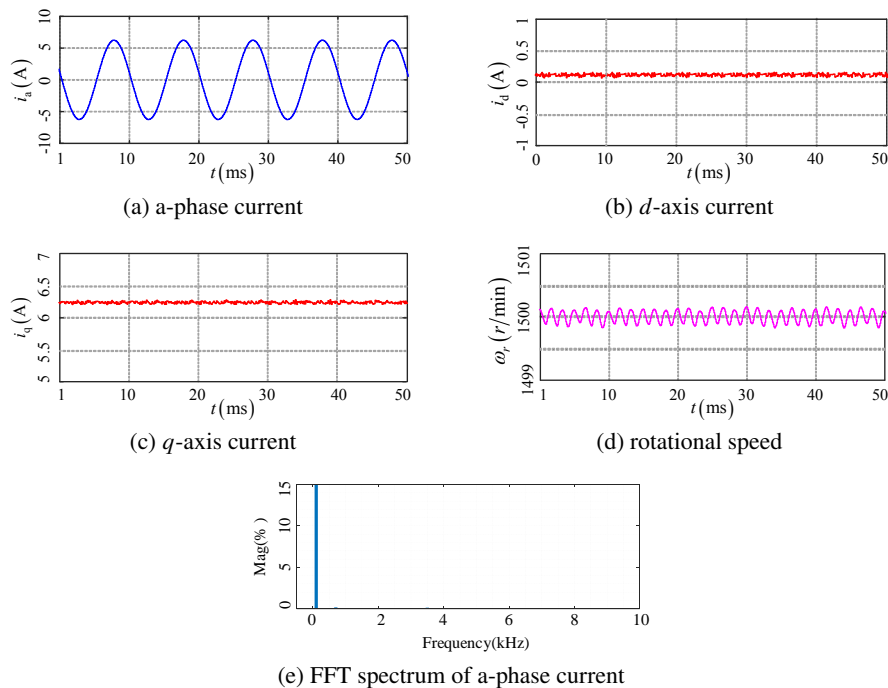
Fig. 6. Experimental waveform of three vector model predictive current control under rated motor parameters
