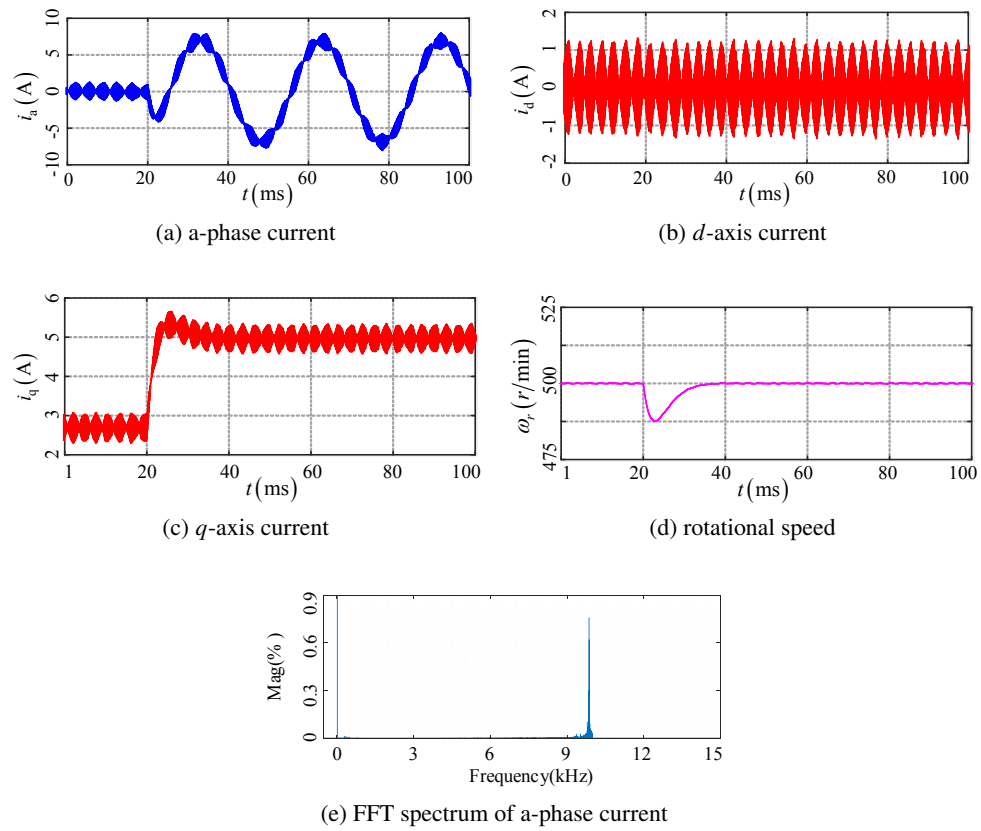
Fig. 10. Experimental waveform of three vector model predictive current control under the condition of motor parameter mismatch
