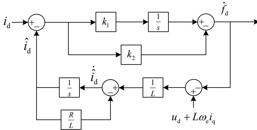
(a) IMC observer of d -axis current
