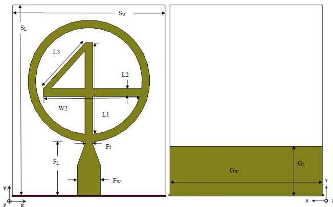
Fig. 6. Proposed ultra-wideband monopole 4-shaped annular ring antenna
