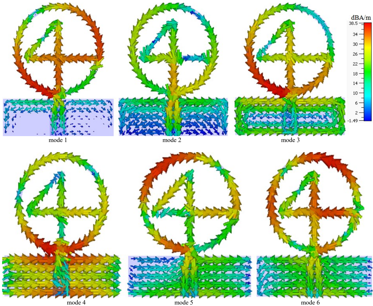
Fig. 4. Distribution of surface currents for modes 1-6 at their resonant frequencies of the proposed model
