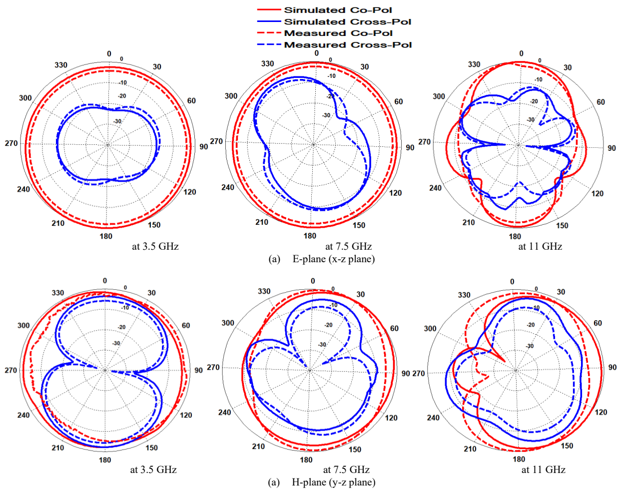
Fig. 9. The 2D radiation patterns of the proposed model at different resonant frequencies.
