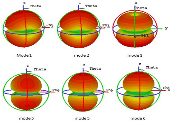
Fig. 5. The 3D modal fields of the 1-6 characteristic modes of the proposed model at their resonant frequencies
