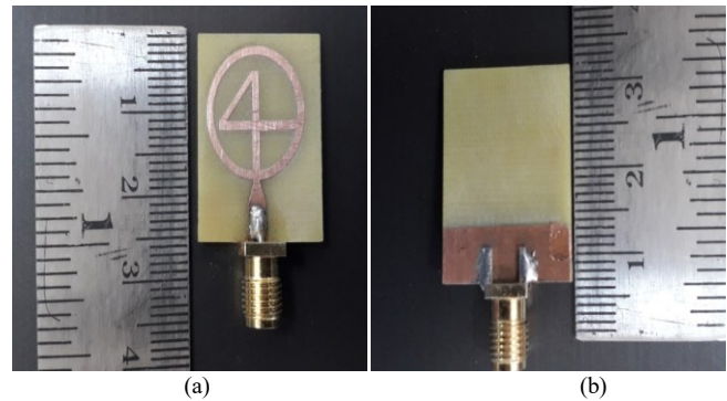
Fig. 7. Photograph of (a) & (b) the top and bottom views of the fabricated antenna.
