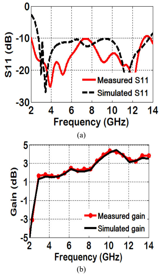
Fig. 8. Proposed antenna measured and simulated (a) S_{11} plot, (b) gain plot
