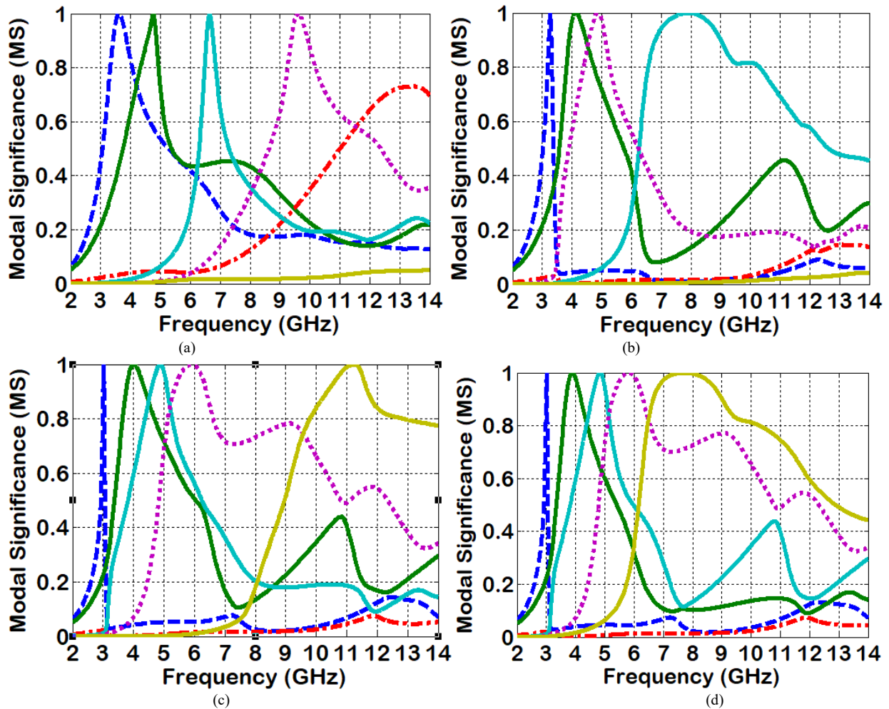
Fig. 3. Modal significance curves of (a) antenna¥1 (b) antenna¥2 (c) antenna¥3 and (d) antenna¥4
