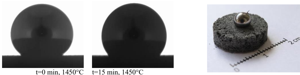
Fig. 3. Photos of the sample - a drop of liquid cast iron in contact with the Magnesia Ceramics | 10 Graphite substrate - during the test of high-temperature wetting kinetics; on the right a photo of the sample after the test
