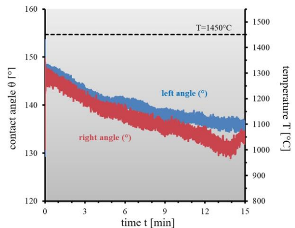
Fig. 5. Wettability kinetics for molten cast iron on Magnesia Ceramics ( \text{Al}_2\text{O}_3 support) substrate under test conditions; CP/15 min/ 1450^\circ\text{C}
