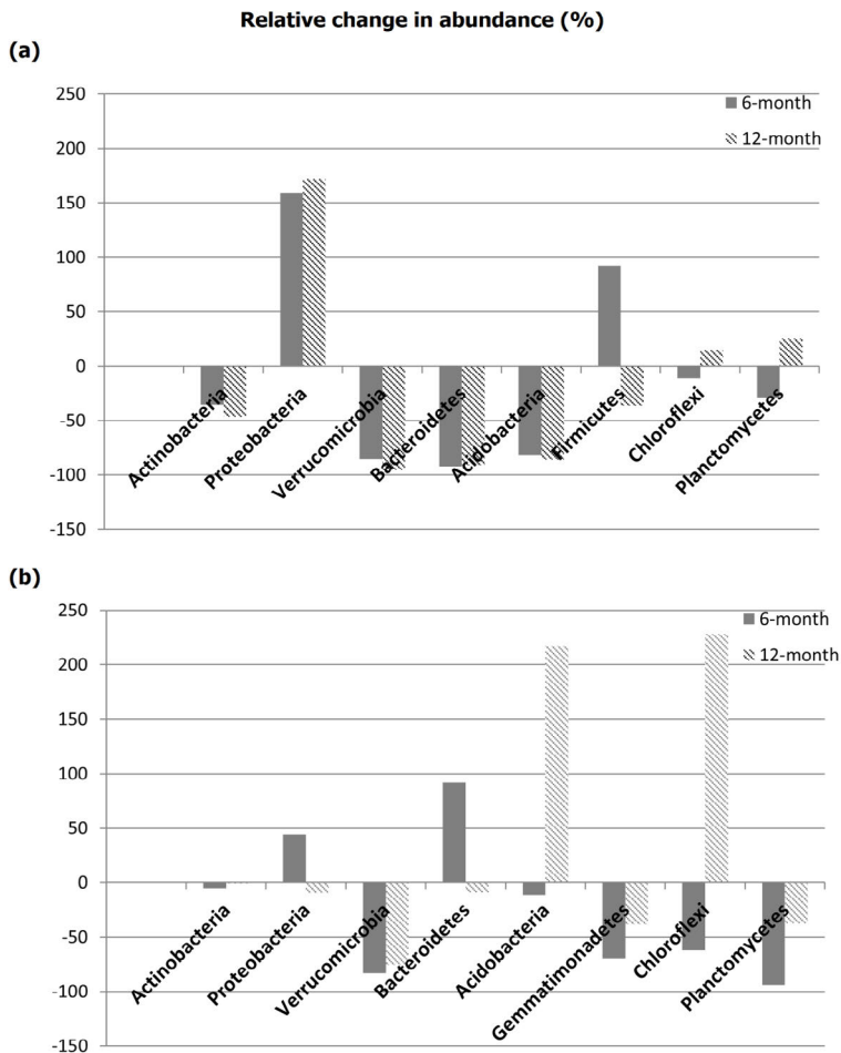
Fig. 4 Relative change in abundance (%) of major bacterial phyla classified in (a) King George Island and (b) Deception Island soil samples at 6 th and 12 th month sampling.
