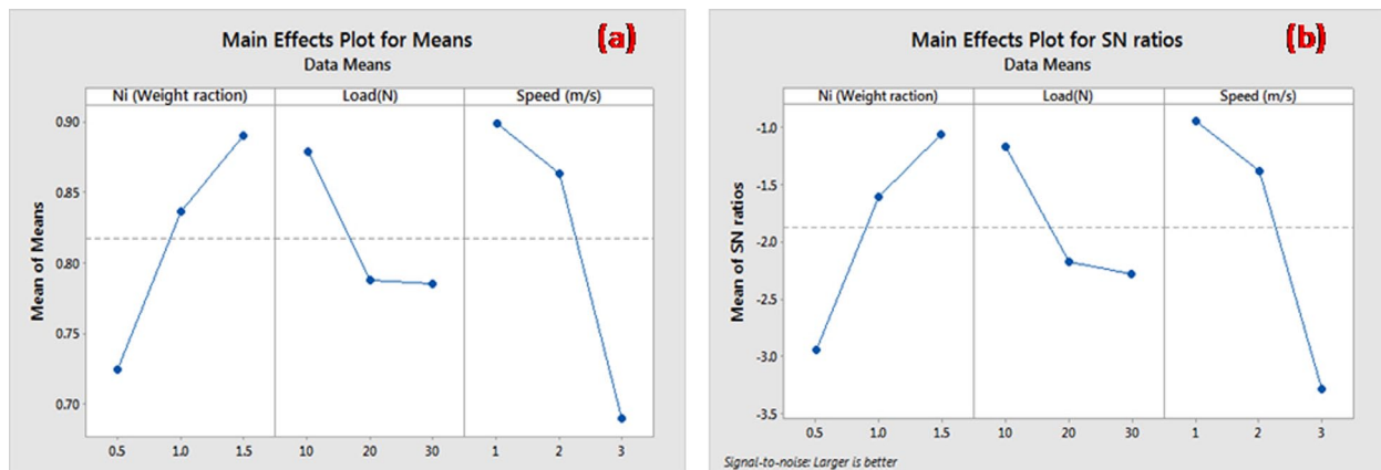
Fig. 9. Main effects plot for (a) mean of CoF (b) mean of S/N ratio of the composites in the peak aged (T6) condition
