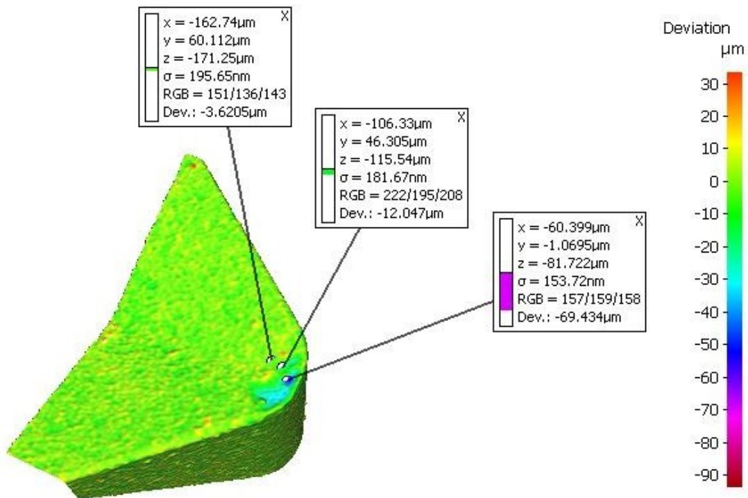
Fig. 8. Height deviation from the reference surface in CT. Deviations are clearly visible by color visualization
