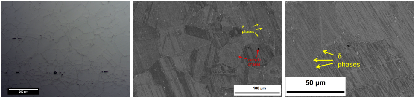
Fig. 1. Microstructure of Inconel 718 at different magnifications
