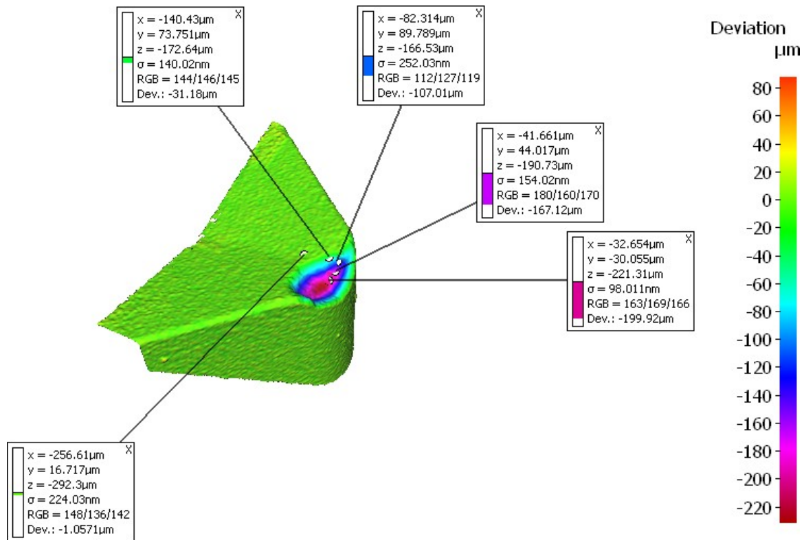
Fig. 9. Height deviation from the reference surface in UAT. Deviations are clearly visible by color visualization
