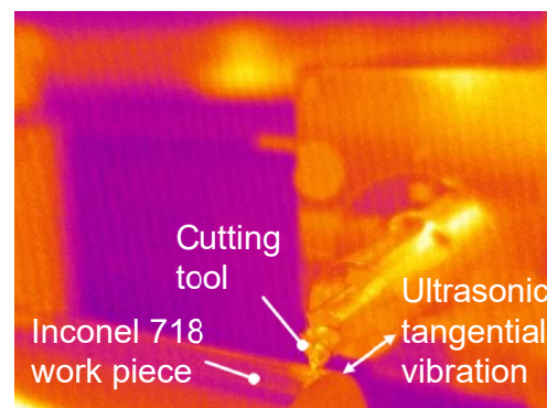
Fig. 2. A schematic diagram of the workpiece along with cutting directions (left), and an image of the cutting tool in ultrasonic tangential vibration (right)
