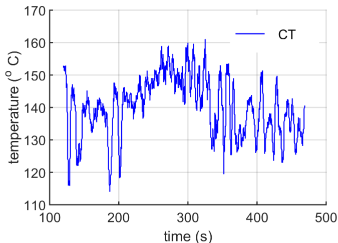
Fig. 5. Average temperature in process zone in CT for Inconel 718
