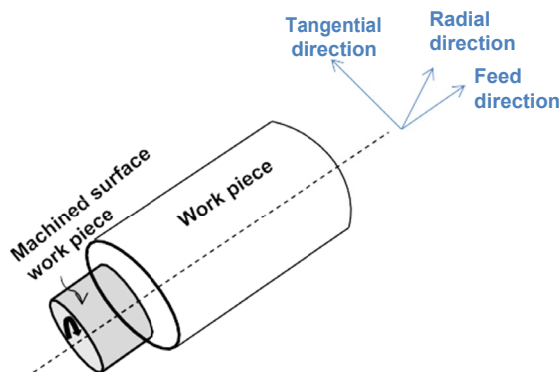
Fig. 2. A schematic diagram of the workpiece along with cutting directions (left), and an image of the cutting tool in ultrasonic tangential vibration (right)
