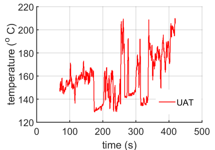
Fig. 6. Average temperature in process zone in UAT for Inconel 718
