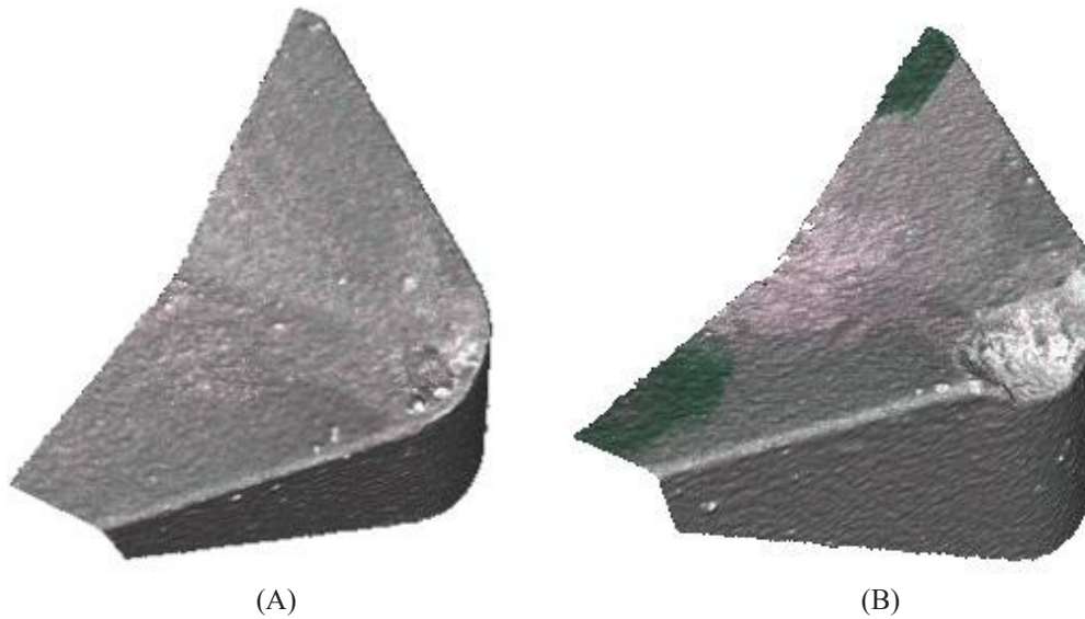
Fig. 7. Tool wear for a 360 s machining period in (A) Conventional turning, and (B) Ultrasonic assisted turning
