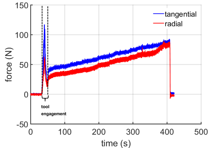
Fig. 4. Tangential and radial force in ultrasonic assisted turning for Inconel 718
