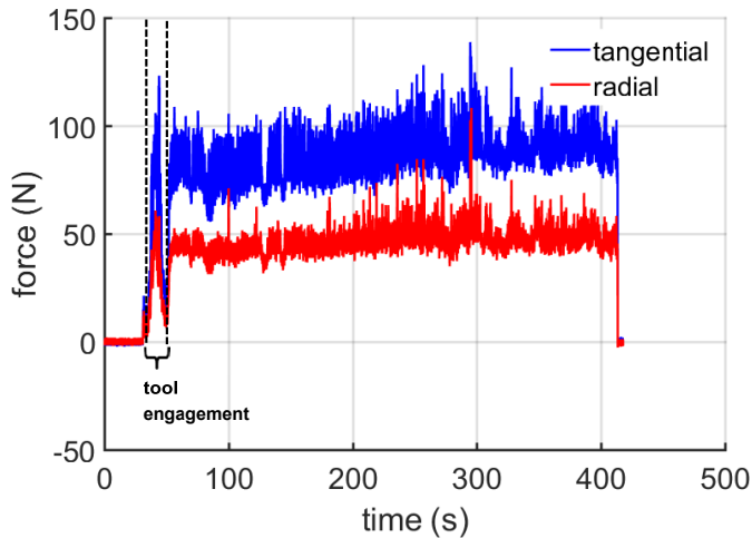
Fig. 3. Tangential and radial force in conventional turning for Inconel 718
