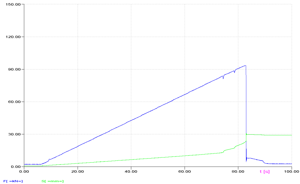
Fig. 5. Tensile force and insulator elongation in the static load strength test 1, tensile load F1 2, elongation E2
