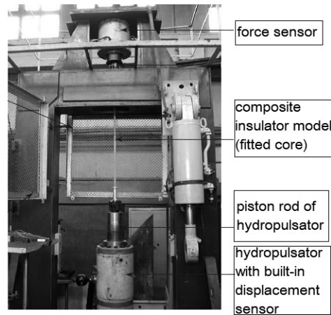
Fig. 4. Test stand with fatigue test-prepared composite insulator model CS 120 C19L 550/3720 for 110 kV line (glass – epoxy resin core without silicone elastomer housing)
