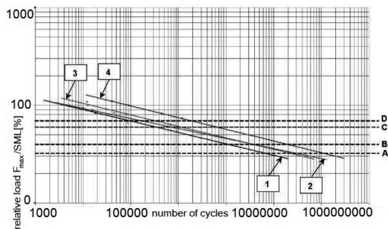
Fig. 8. Fatigue characteristics of composite insulators, determined for selected values of amplitudes of cyclic load changes (logarithmic scale on both axes): characteristic for amplitude F_a = 25\%F_m , characteristic for amplitude F_a = 20\%F_m , characteristic for amplitude F_a = 5\%F_m , characteristic for amplitude F_a = 10\%F_m
