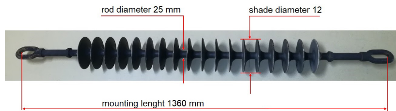
Fig. 2. Composite insulator removed from the line after 35 years of operation
