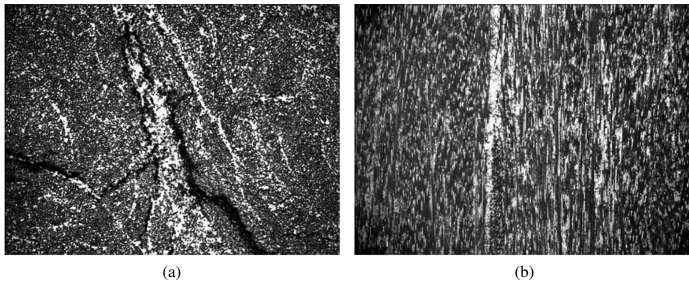
Fig. 7. Microscopic photographs of samples taken from the core of the composite insulator from Fig. 2 after a destructive static load test (magnification \times 50 ): (a) cracks observed at the cross-section area; (b) cracks observed on the surface of the right section
