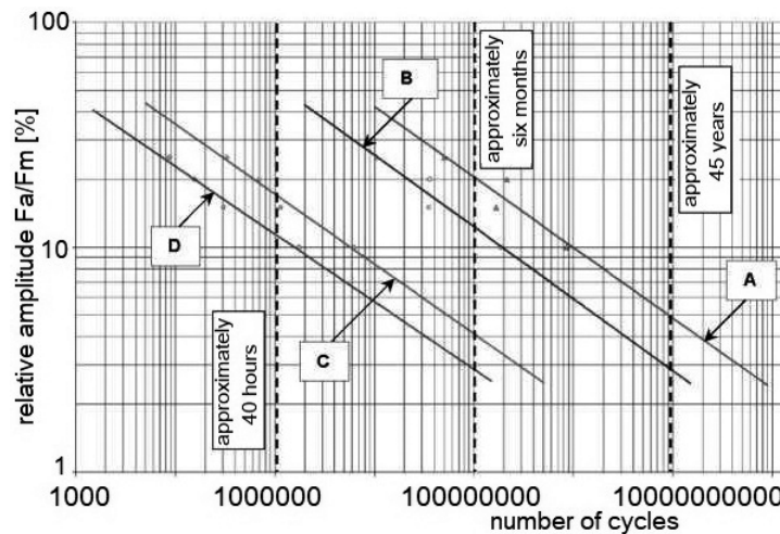
Fig. 9. Fatigue characteristics of composite insulators, determined for four values of maximum cyclic tensile load (logarithmic scale on both axes): F_{\max} = 33.3\% SML, F_{\max} = 40.0\% SML, F_{\max} = 60.0\% SML, F_{\max} = 70.0\% SML
