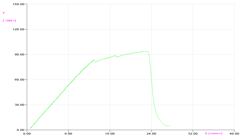
Fig. 6. Relationship between elongation and tensile load for insulator from Fig. 2 in mechanical strength test under static load
