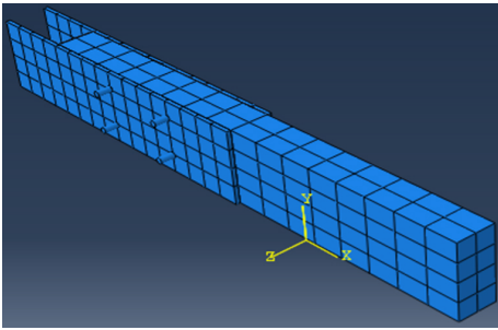
Fig. 7. Assembled model
