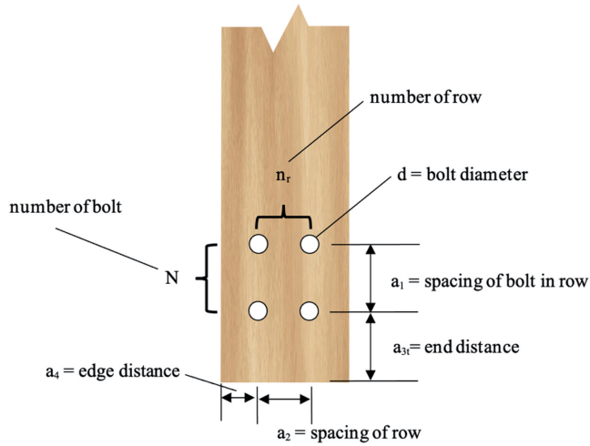
Fig. 6. Definitions of the variables used [12]
