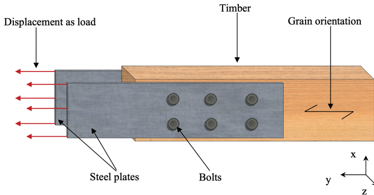
Fig. 1. Steel-wood-steel connection loaded parallel to grain [12]
