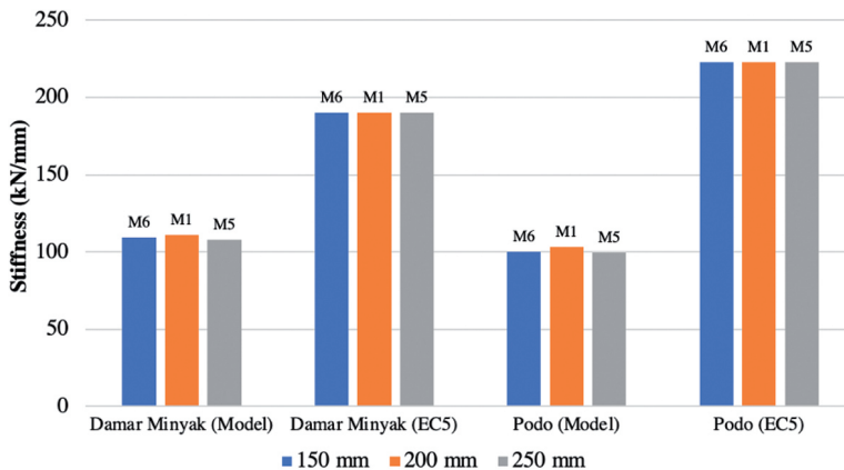
Fig. 17. Stiffness versus bolt spacing
