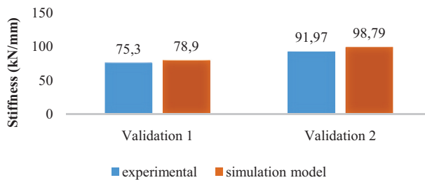
Fig. 12. Comparison of experimental and simulation model
