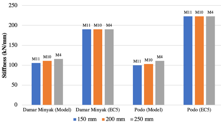
Fig. 16. Stiffness versus end distance
