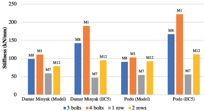
Fig. 18. Stiffness versus number of bolts and rows
