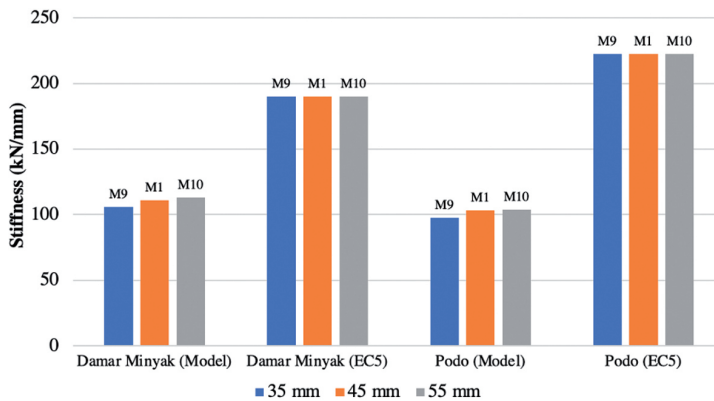
Fig. 19. Stiffness versus edge distance
