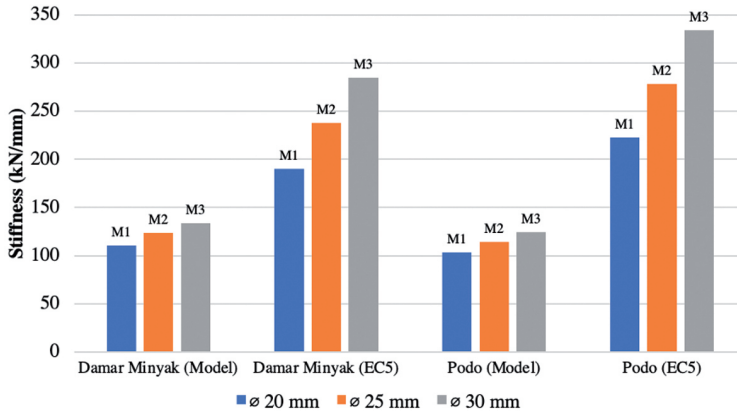
Fig. 15. Stiffness versus bolt diameter
