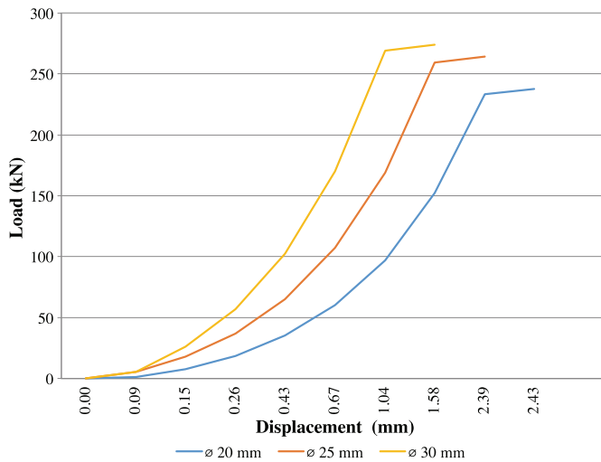
Fig. 14. Load versus displacement graph for Podo with various bolt diameters
