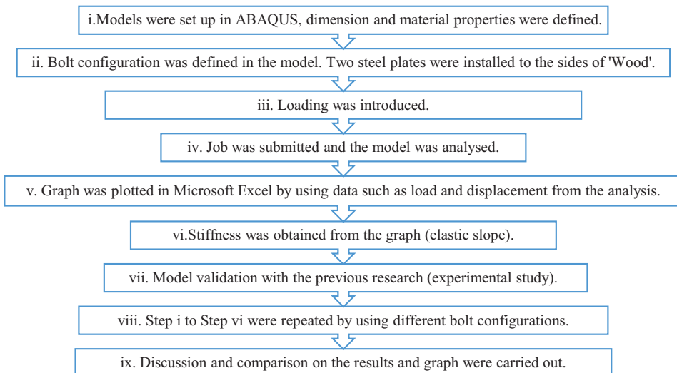
Fig. 2. Finite element analysis flowchart for bolted timber connection
