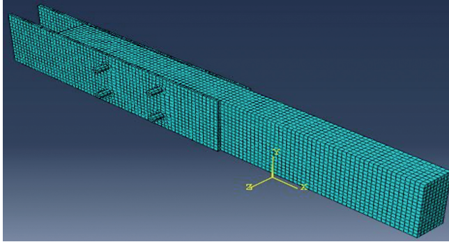
Fig. 9. Meshed model
