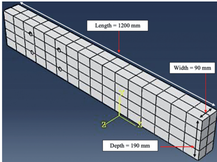
Fig. 3. Model for timber
