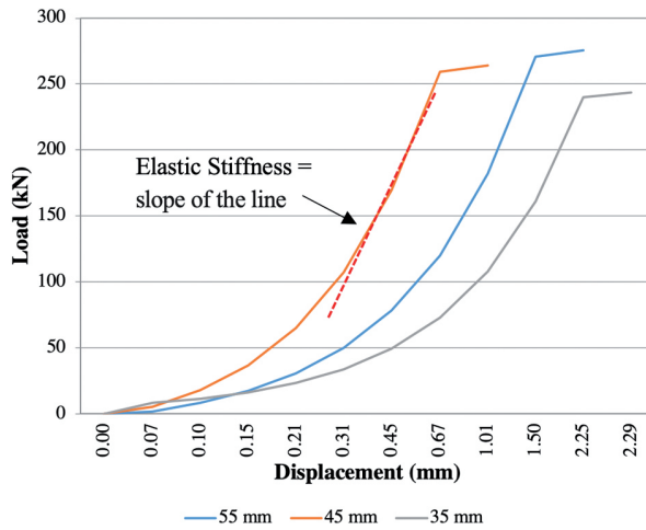
Fig. 13. Load versus displacement graph for Damar Minyak with various edge distance
