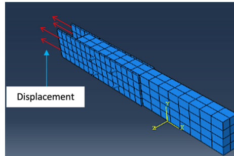
Fig. 8. Displacement control as load
