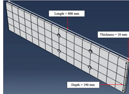
Fig. 4. Model for steel plate
