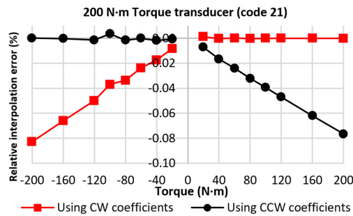
Fig. 4. Cubic relative interpolation error for the 200 N·m torque transducer (Code 21).
