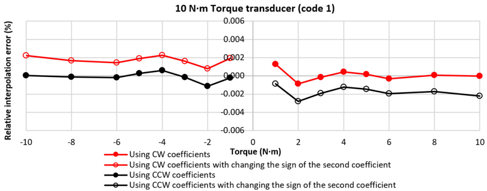
Fig. 12. Cubic relative interpolation errors for the 10 N·m torque transducer (Code 1) by applying (1) and (3).
