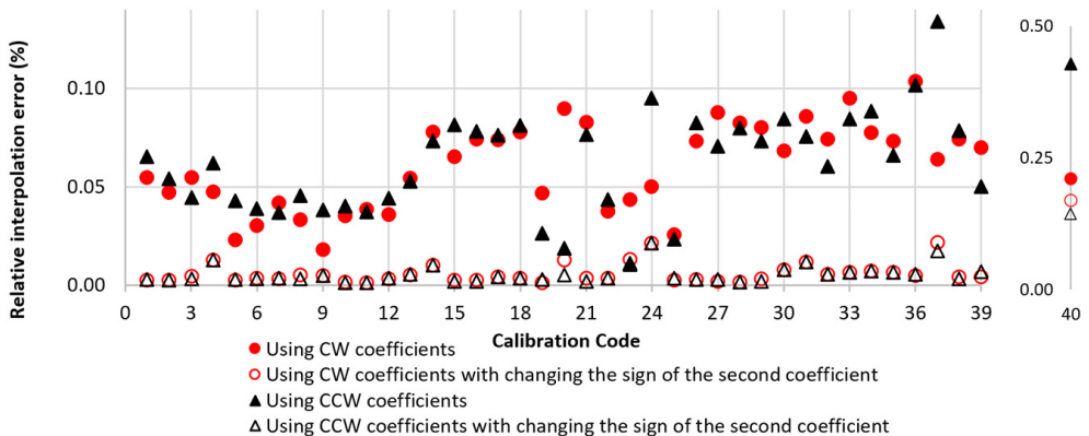
Fig. 19. Maximum relative interpolation error of the 40 calibrations by applying Equations (1) and (3). Note: Code 40 has a different scale.
