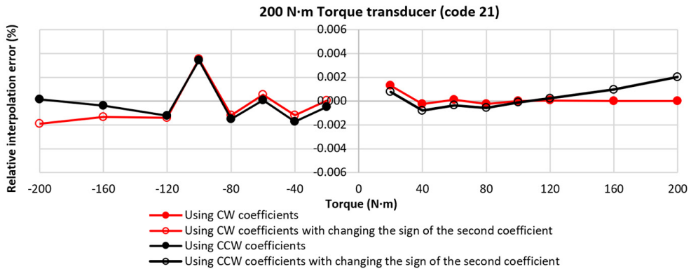
Fig. 14. Cubic relative interpolation errors for the 200 N-m torque transducer (Code 21) by applying (1) and (3).
