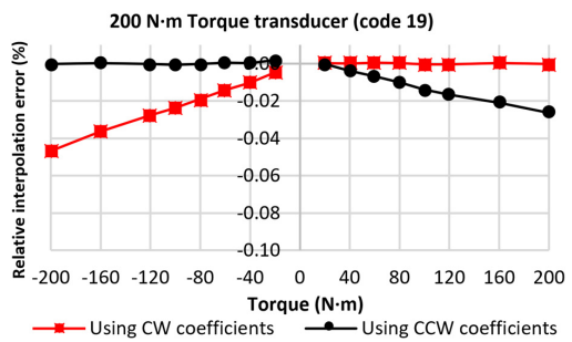
Fig. 3. Cubic relative interpolation error for the 200 N·m torque transducer (Code 19).
