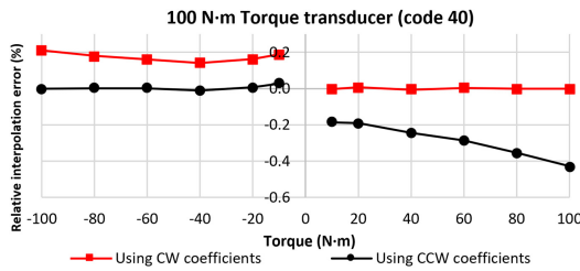
Fig. 8. Cubic relative interpolation error for the 100 N·m torque transducer (Code 40).
