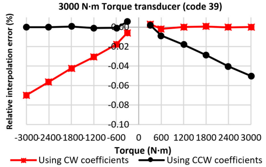
Fig. 7. Cubic relative interpolation error for the 3000 N·m torque transducer (Code 39).
