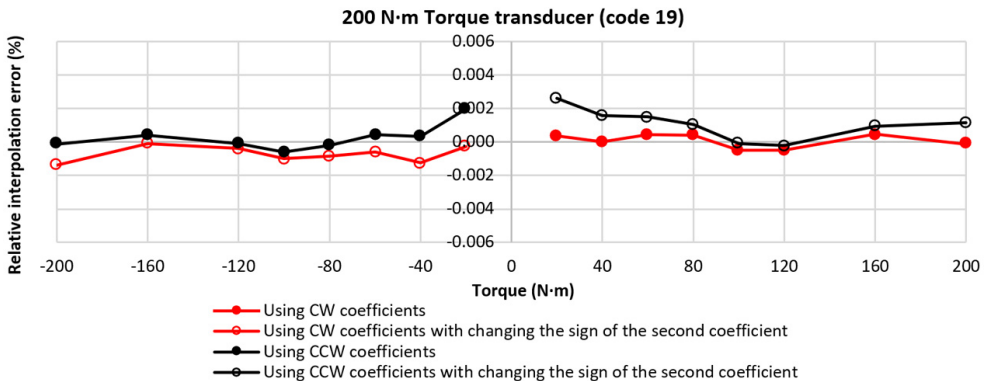
Fig. 13. Cubic relative interpolation errors for the 200 N·m torque transducer (Code 19) by applying (1) and (3).
