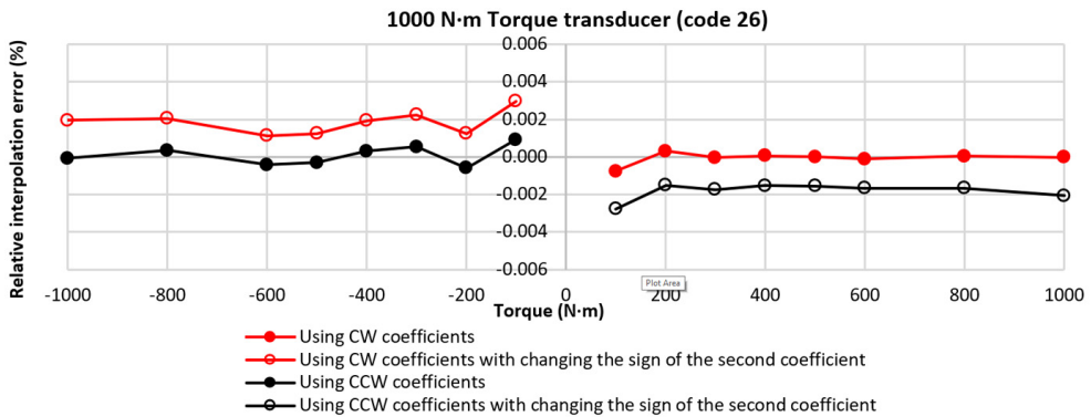
Fig. 15. Cubic relative interpolation errors for the 1000 N-m torque transducer (Code 26) by applying (1) and (3).
