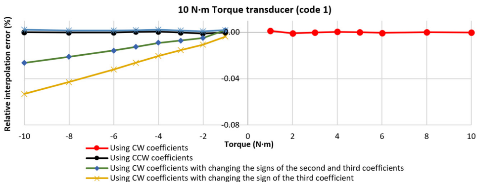
Fig. 10. Relative interpolation errors calculated by different models for the 10 N·m torque transducer (Code 1).
