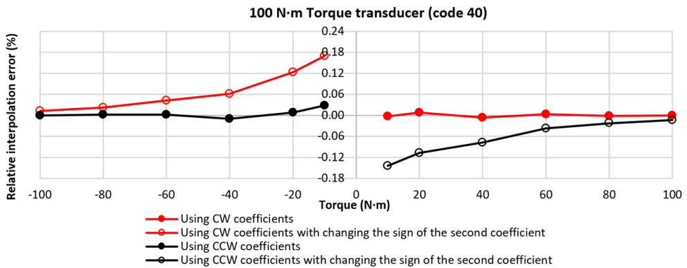
Fig. 18. Cubic relative interpolation errors for the 100 N·m torque transducer (Code 40) by applying (1) and (3).
