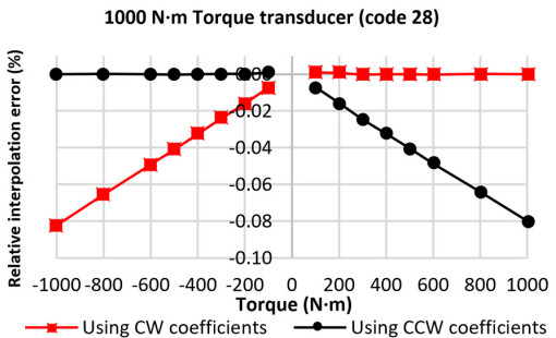
Fig. 5. Cubic relative interpolation error for the 1000 N·m torque transducer (Code 28).
