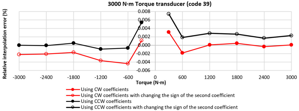
Fig. 17. Cubic relative interpolation errors for the 3000 N·m torque transducer (Code 39) by applying (1) and (3).
