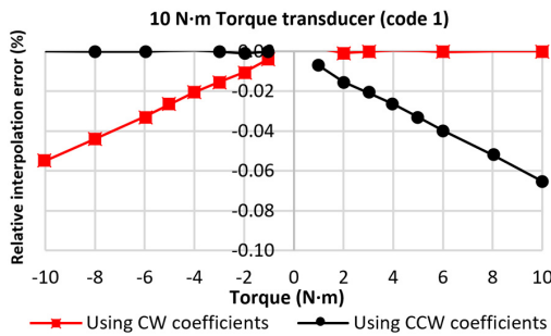
Fig. 2. Cubic relative interpolation error for the 10 N·m torque transducer (Code 1).
