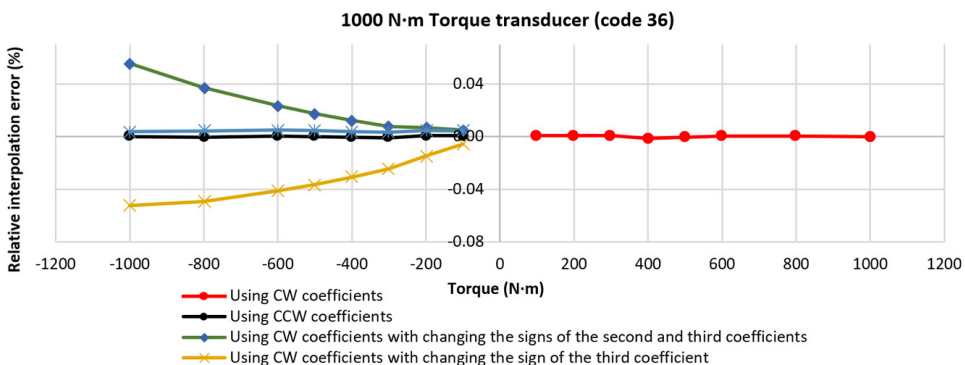
Fig. 11. Relative interpolation errors calculated by different models for the 1000 N·m torque transducer (Code 36).
