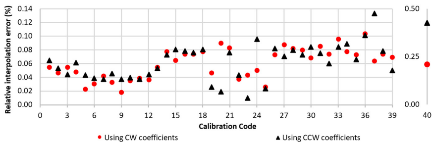
Fig. 9. Maximum relative interpolation error of the 40 calibrations. Note: Code 40 has a different scale.
