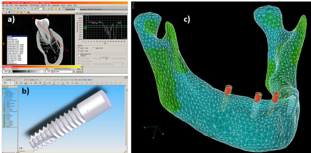
Fig. 9. Planning an implantoprosthodontic procedure based on CBCT with the use of FEM: a) distribution of bone density in the area of implant application along the indicated line, b) virtual implant, c) model of the mandible with the arrangement of implants.
