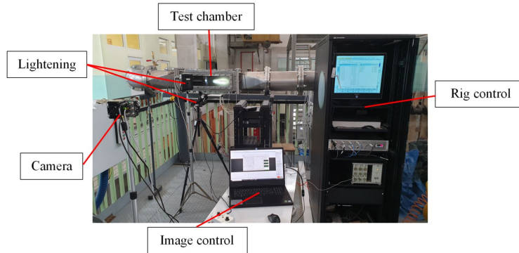
Figure 4: The measuring system including a high-speed camera, image control, rig control, lightening and test chamber.
