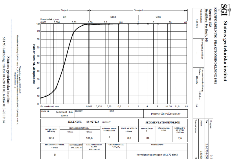
Fig. 2. The grain distribution diagram for aggregated sample collected from the site B6b. The laboratory tests of soil sieve analysis and curve plotting were performed at the SGI by Per Lindh
