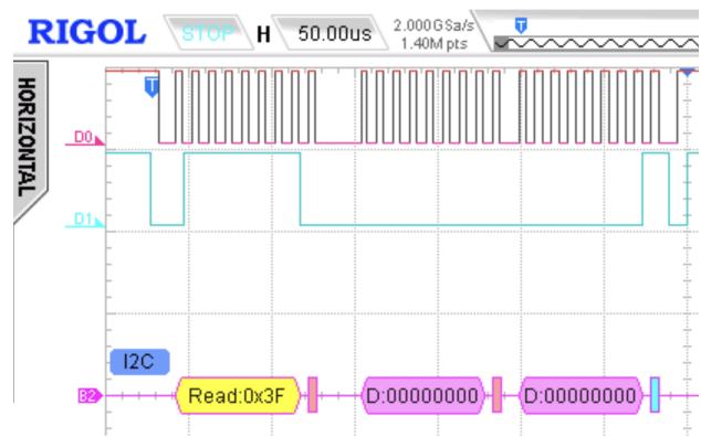
Fig. 10. Example of an I 2 C frame measurement taken without light source.
