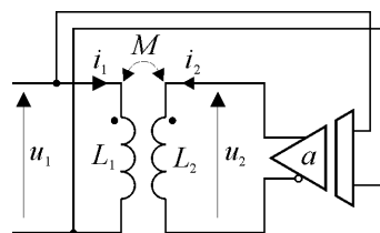
Fig. 8. Diagram of a inductor circuit with a true smooth value of the equivalent inductance
