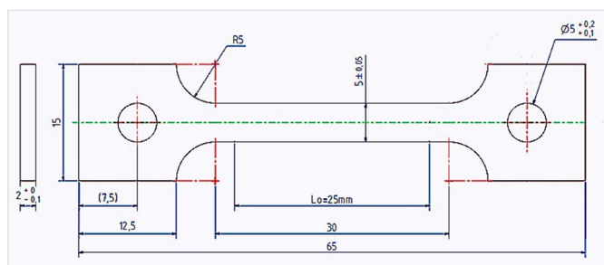
Fig. 2. Dimensional size of the sample for tensile testing
