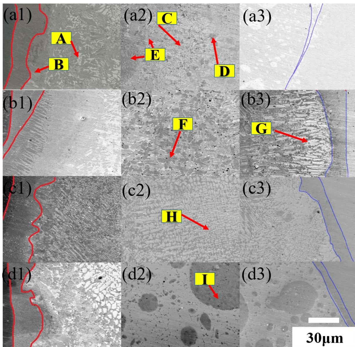
Fig. 7. SEM analysis of the joint microstructure under the condition of different laser power: (a) 2100 W, (b) 2300 W, (c) 2500 W, (d) 2700 W, and the number 1,2,3 respectively represented the weld zone near the TA15, the weld center and the weld zone near Inconel 718
