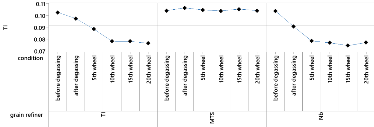
Fig. 4. Change in Ti content by casting sequence
