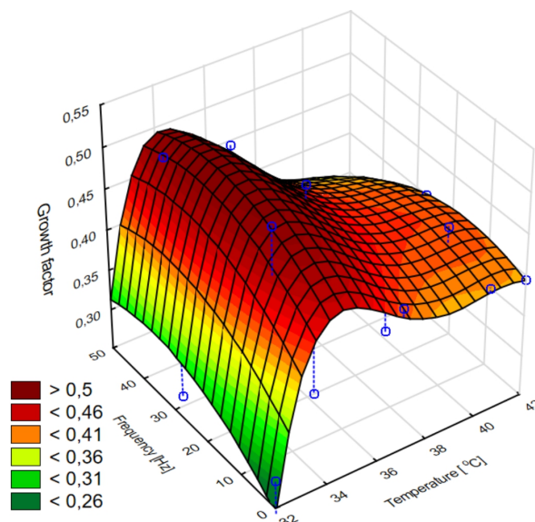
Fig. 5. Surface plot of the adjusted growth factor \phi(T, f) function to the experimental data
