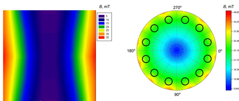
Fig. 2. Typical distribution of magnetic flux density in the RMF generator: a) vertical cross-section, b) horizontal cross-section at the position of the samples ( f = 30 Hz)
