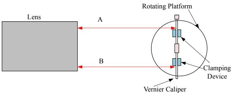
Fig. 13. Sketch diagram of parallelism adjustment.
