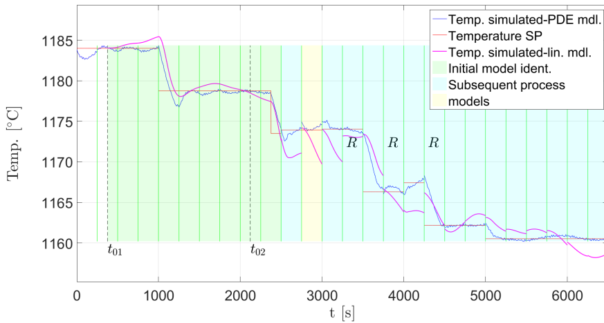
Figure 9: Simulated temperature in the third zone of the forehearth – the second experiment
