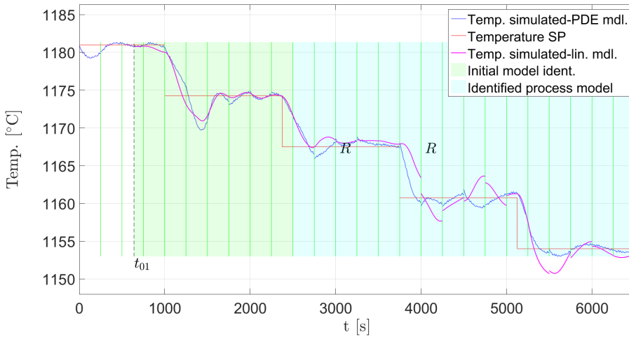
Figure 11: Simulated temperature in the fourth zone of the forehearth – the second experiment
