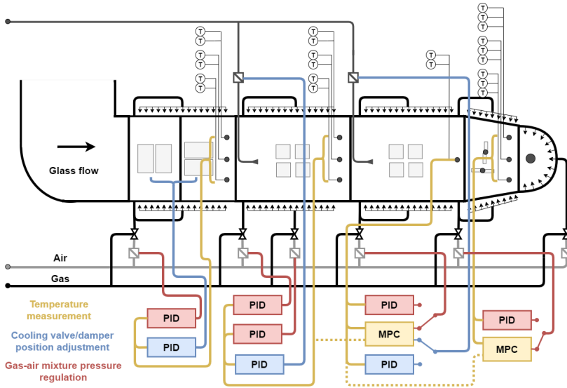
Figure 1: Control system of a glass forehearth
