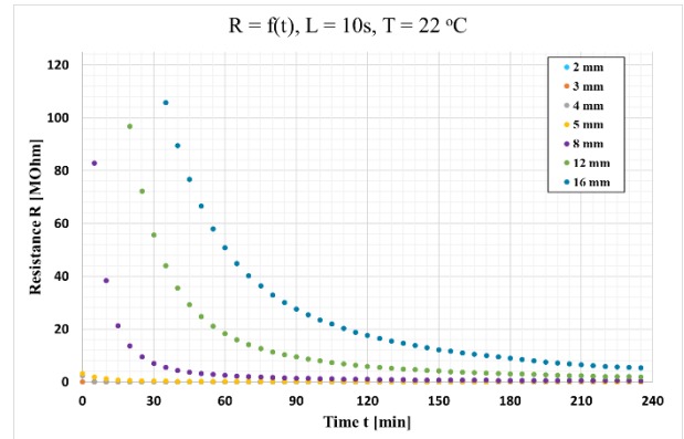
Fig. 7. Process of moisture sorption in the surface layer of the sand mould, L = 10\text{ s} , T = 22\text{ }^{\circ}\text{C}
