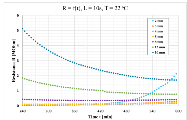
Fig. 8. Transition phase of the moisture migration process in the surface layer of the sand mould, L = 10\text{ s} , T = 22\text{ }^{\circ}\text{C}
