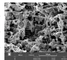
Fig. 5. Detail of a micro-shrinkage
