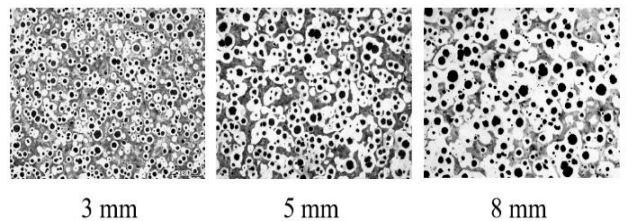
Fig. 10. Structure of 3, 5 and 8 mm thick castings
