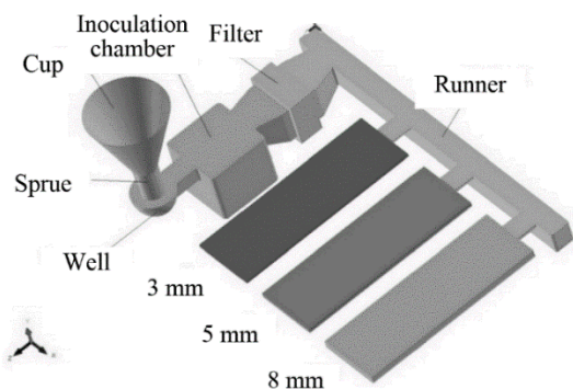
Fig. 2. Scheme of the experimental castings
