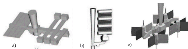
Fig. 1. Test pieces a),b) by Stefanescu, c) by Labresque [4, 15]
