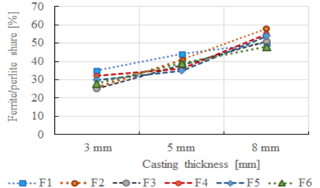
Fig. 11. Ferrite/pearlite proportion in the structure
