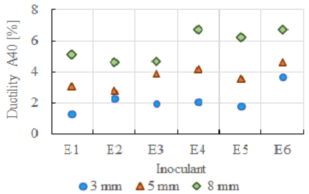
Fig. 15. Relation of the ductility on the casting thickness
