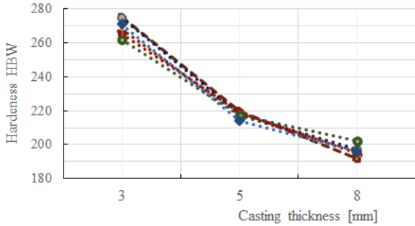
Fig. 12. Influence of the casting wall thickness and inoculant type on hardness
