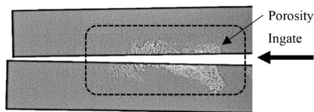
Fig. 3. X-ray image of an internal shrinkage in a casting thick 3 mm
