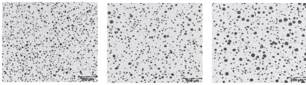
Fig. 6. Graphite in samples thick 3, 5, and 8 mm
