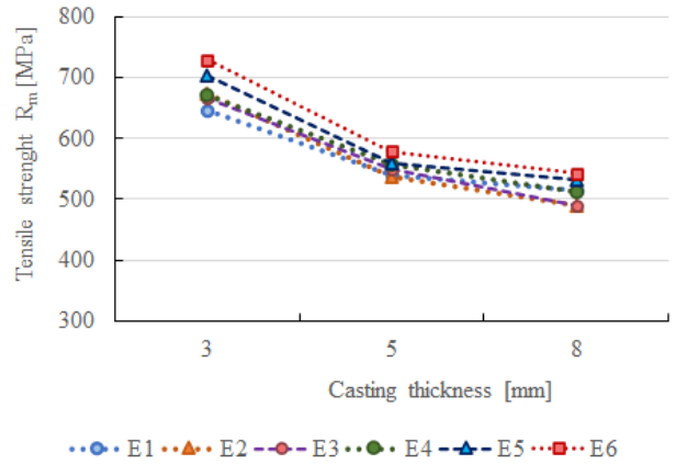
Fig. 14. Relation of the tensile strength on the casting thickness
