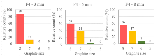
Fig. 7. Graphite size in castings from melt F
