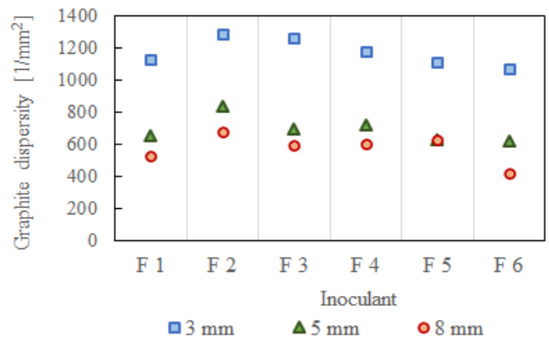
Fig. 9. Influence of the inoculants on the graphite dispersity
