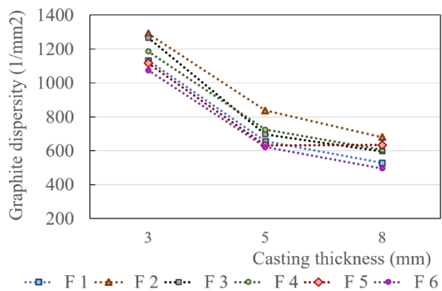
Fig. 8. Graphite dispersity depending on the casting wall thicknesses
