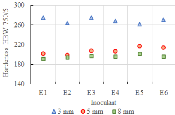
Fig. 13. Relation of hardness on the inoculant type
