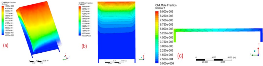
Fig. 6. Gas concentration distribution map at a horizontal distance of 25 m and a vertical height of 35 m in a high level roadway. (a) Stereoscopic plot of gas concentration distribution at a vertical distance of 35 m, (b) Gas concentration slice plot at z = 1.7 m, (c) Mining face gas concentration slice plot
