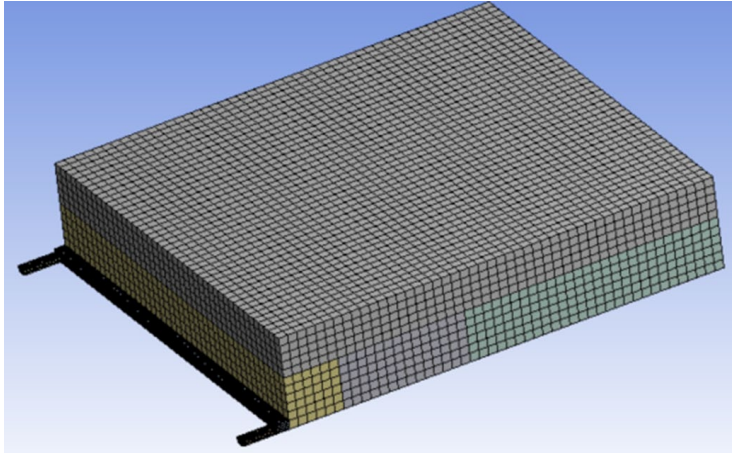
Fig. 3. Grid division of the physical model of the mining area of the mining face
