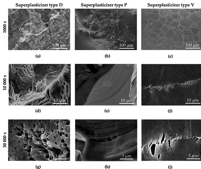
Fig. 4. SEM sectional images for superplasticizers type D, type P, type V in various magnifications
