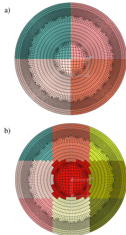
Fig. 5. Division of the reservoir foundation area into a) four (Case 2) and b) nine sub-areas (Case 3)
