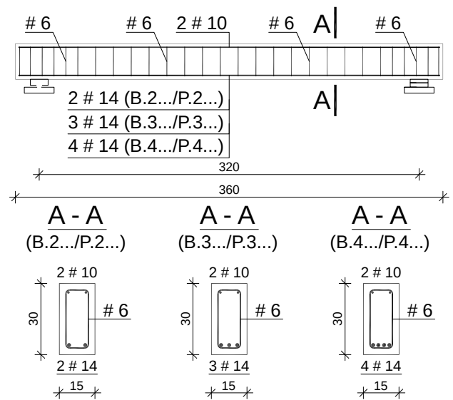
Fig. 1. Dimensions and arrangement of rebars in the RC beams (dimensions in cm)
