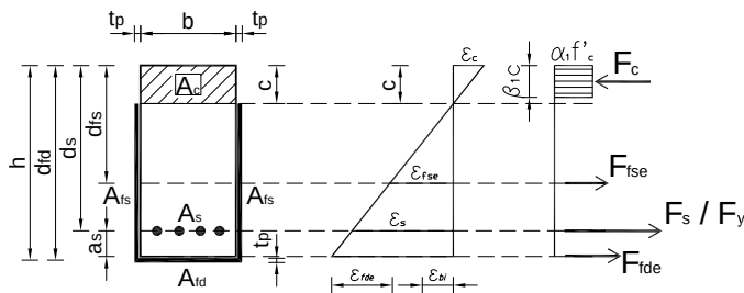
Fig. 12. Internal strain and stress distribution model for a rectangular section under flexure at ultimate limit state (ULS) for beam with polyurea coating
