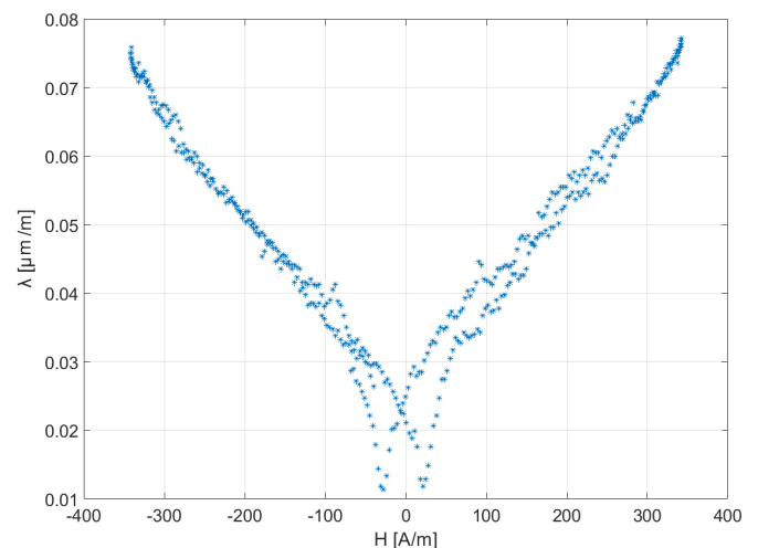
Fig. 8. Magnetostrictive hysteresis loop for the amorphous 2605Co ribbon attached to the piezoelectric material PZ27
