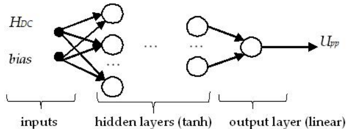
Fig. 17. Structure of the MLP applied to model the output characteristics of the sensor
