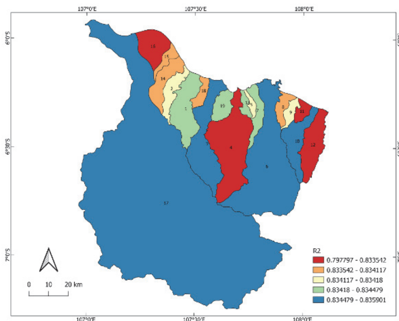
Fig. 5. The Local R 2 of the GWR model
