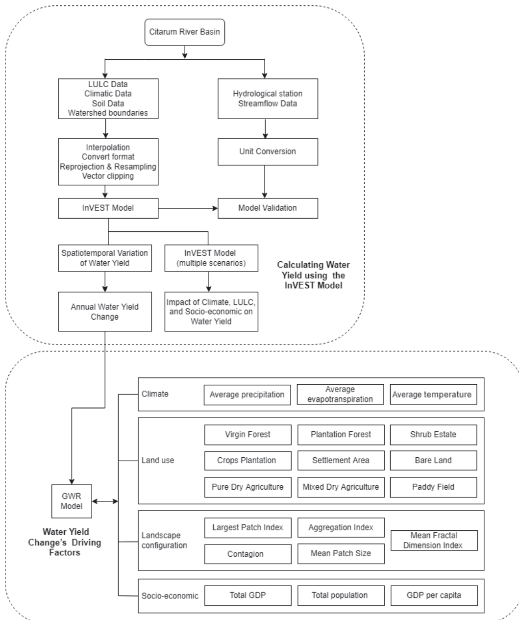
Fig. 2. Research flowchart
