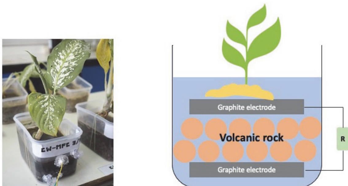
Fig. 1. The diagram of CW-MFC with macrophyte on a cathodic electrode
