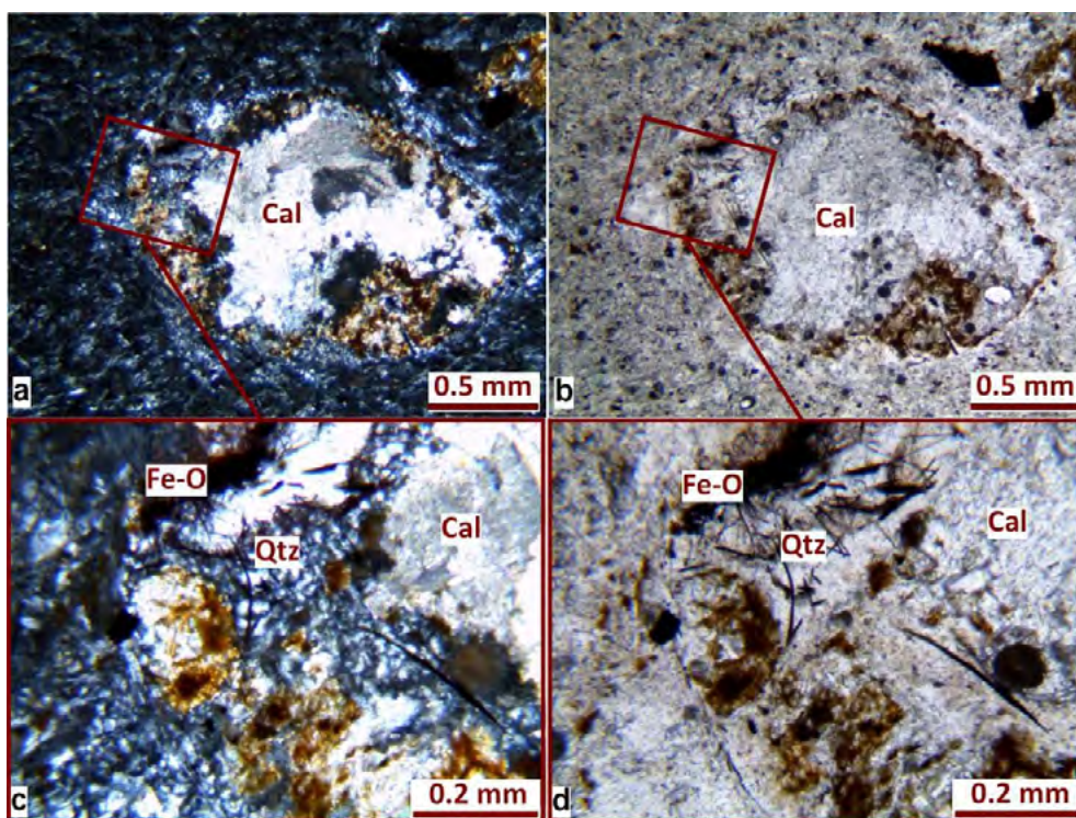
Fig. 5. Silica minerals replacing calcite minerals in iron-oxide-calcite filled pores in volcanic host rocks
