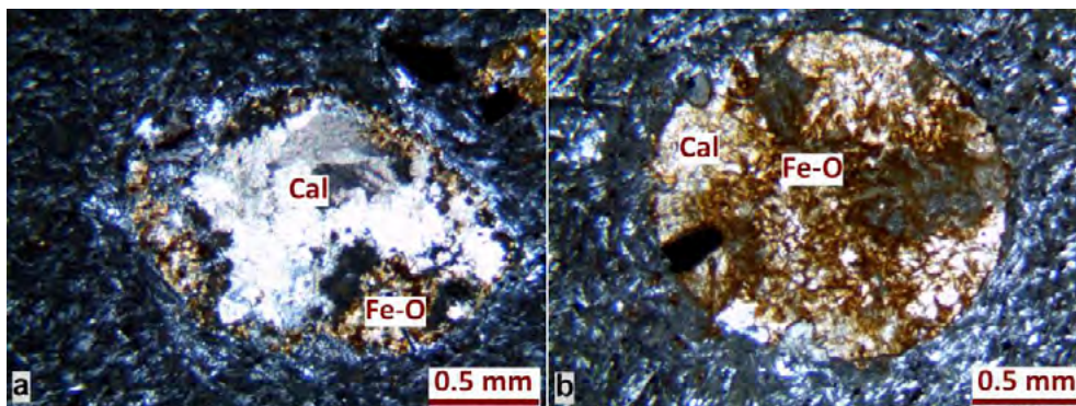
Fig. 4. Iron oxide and calcite filling formed in pores in volcanic host rocks
