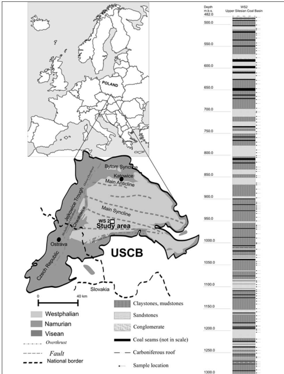
Fig. 1. Schematic of the Upper Silesian Coal Basin and location of the study area (modified from Jureczka and Kotas 1995; Kędzior 2015) with a simplified profile of the Westphalian for the Upper Silesian Coal Basin
