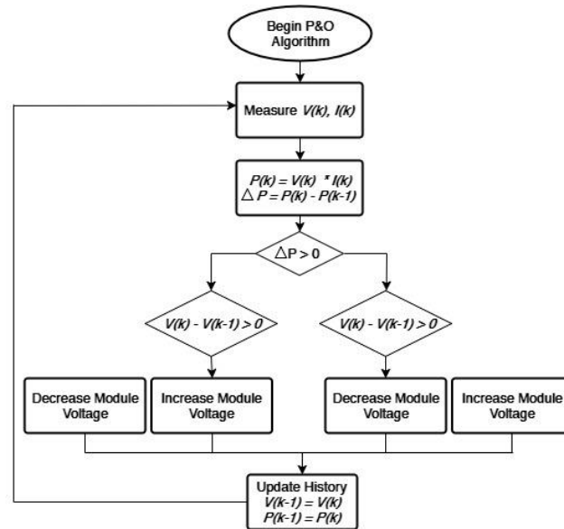
Fig. 10. Flowchart P&O
