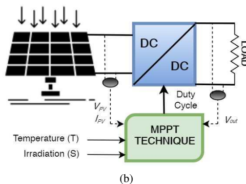
Fig. 5. Parametric temperature methods: (a) flowchart and (b) block diagrams
