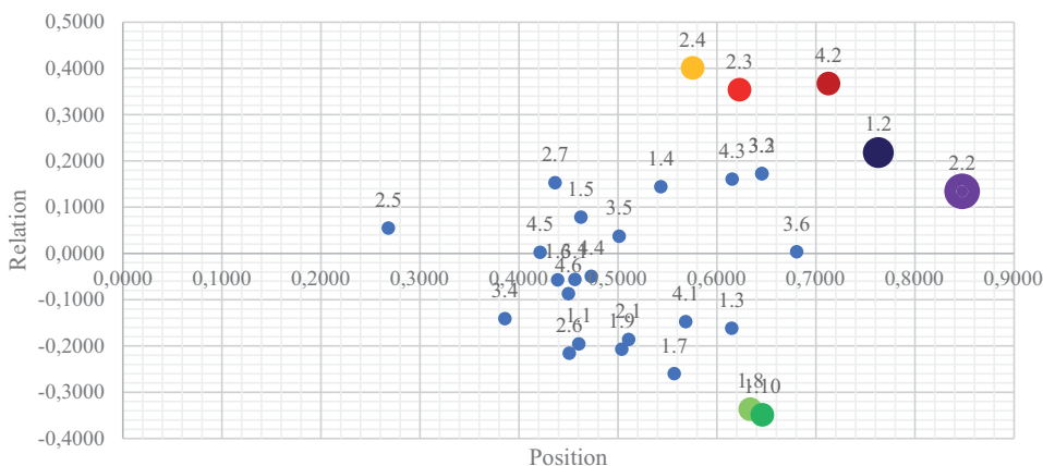
Fig. 3. Graphical interpretation of DEMATEL results
