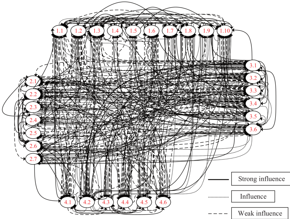
Fig. 1. Direct influence graph – expert evaluation results
