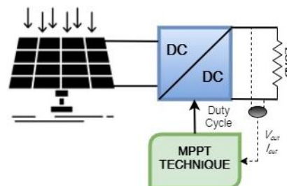
Fig. 9. Schematic of the Load Voltage/Load Current Maximization method
