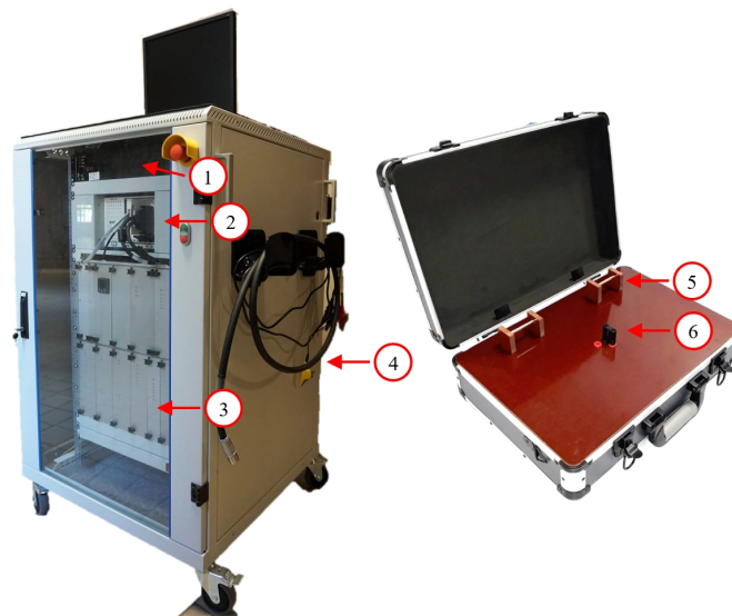
Fig. 5. Front-right view of the capacitor discharge diagnostic system unit (left) and SC winding simulator (right): 1 – control computer, 2 – NI PXI chassis with NI PXI remote control module, NI PXI DAQ card and NI PXI DIO card, 3 – main capacitor bank, 4 – test leads, 5 – HV test leads connection points, 6 – banana jumper for CDS configuration
