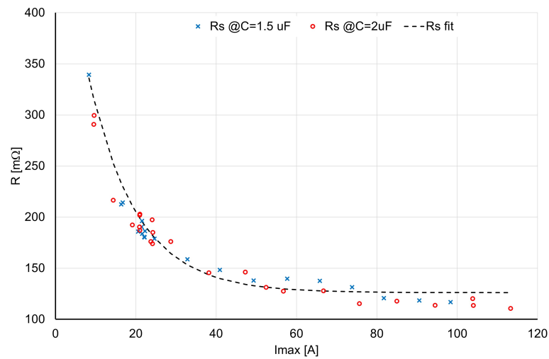
Fig. 11. Resistance of the CDDS as a function of maximum discharge current, determined from measurements for different capacitance values
