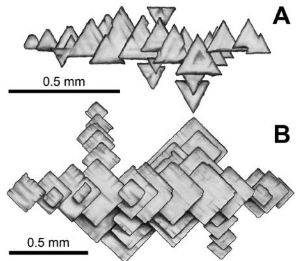
Text-fig. 9. Native silver crystals of octahedral habit developed according to the face \{111\} , Lwia Mt. (A) and crystals of square plate habit with the face \{100\} as the main one, Płonik Mt. (B).
