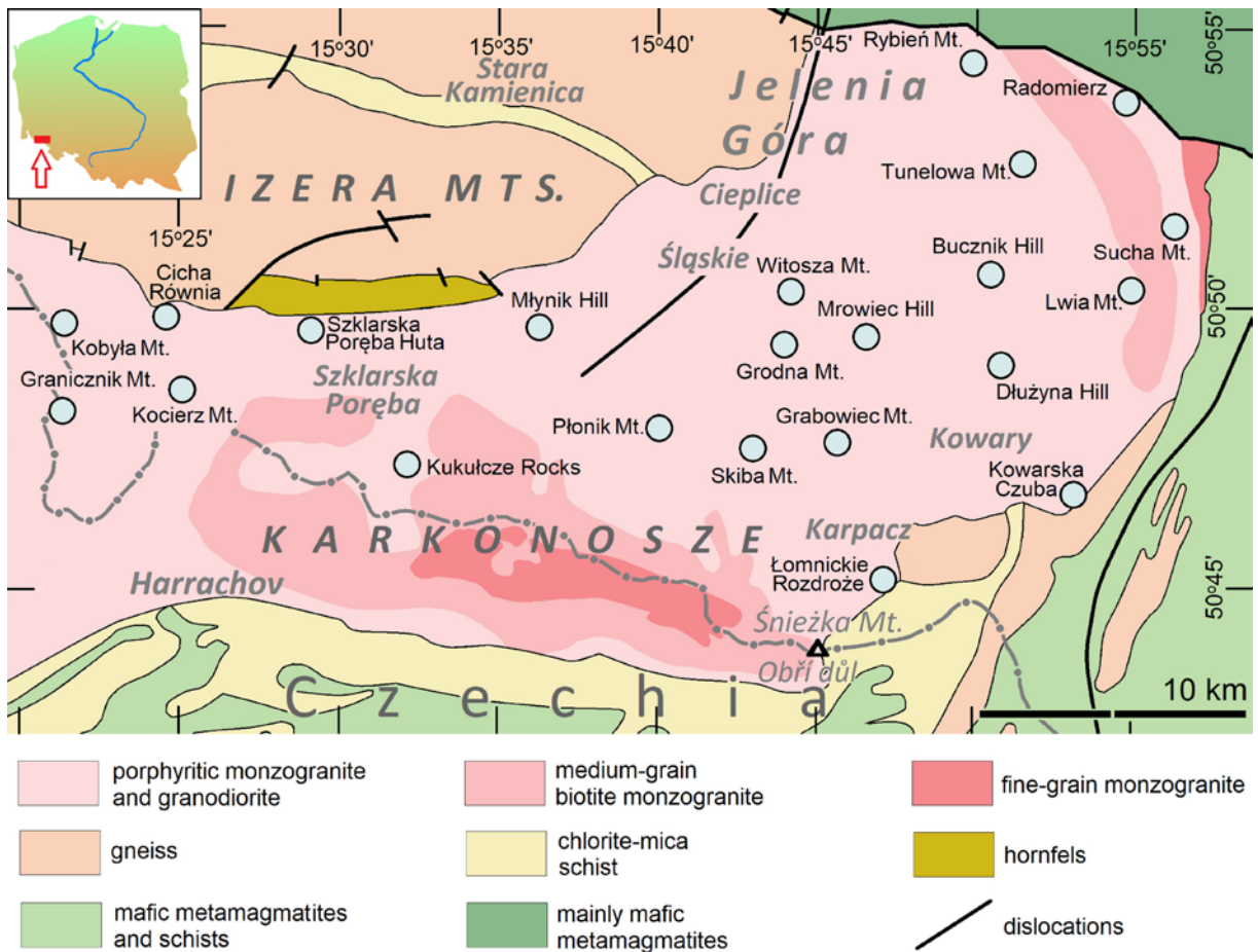
Text-fig. 1. Eastern part of the Karkonosze Variscan granitoid pluton and its metamorphic envelope; circles – sampling locations of the native silver specimens. Geological background after Krenz et al. (2001), changed. Insert – location in Poland.
