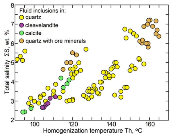
Text-fig. 18. The plot: homogenization temperature vs. total salinity of primary fluid inclusions in host minerals of silver; each circle marks one inclusion.
