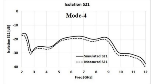
Fig. 9. Comparison between simulated and measured S-parameters (S21)
