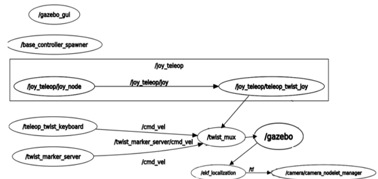
Fig. 2. ROS Node Diagram Proposed
