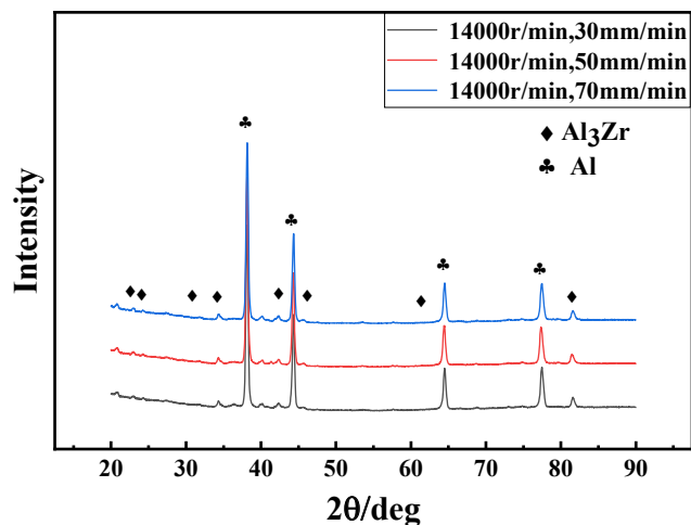
Fig. 8. XRD patterns of FSW joints with different welding parameters
