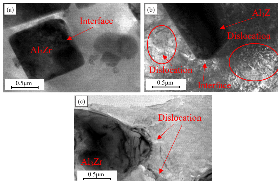
Fig. 11. TEM micrograph of FSW joint. (a) Reinforcing particles; (b-c) Interface between reinforcement particles and matrix
