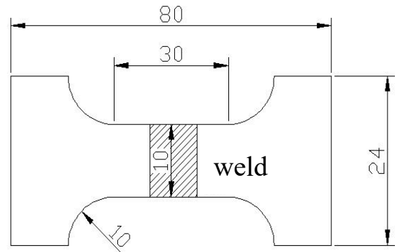
Fig. 3. Schematic diagram of tensile specimen size
