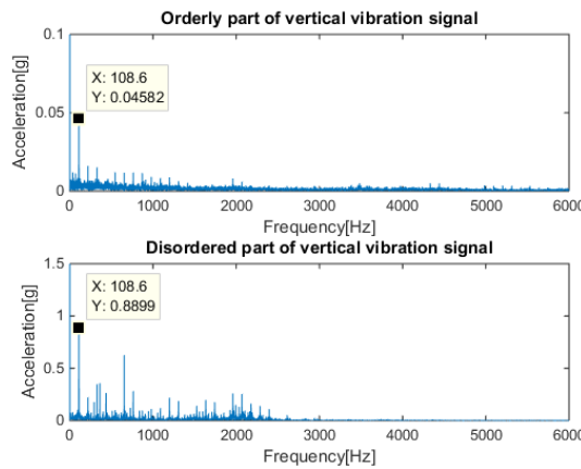
Fig. 9. Envelope spectrum of vertical signal
