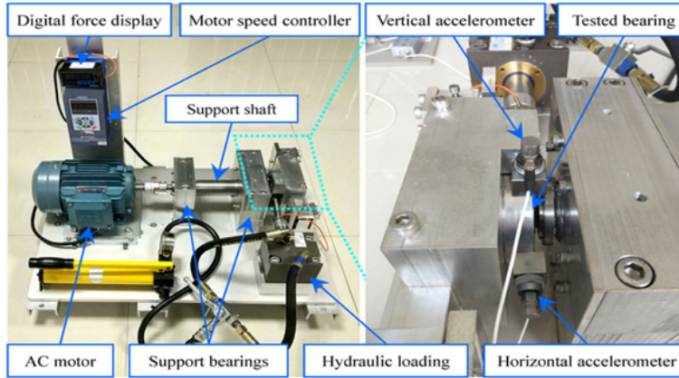
Fig. 3. Test strip used in the XJTU-SY database
