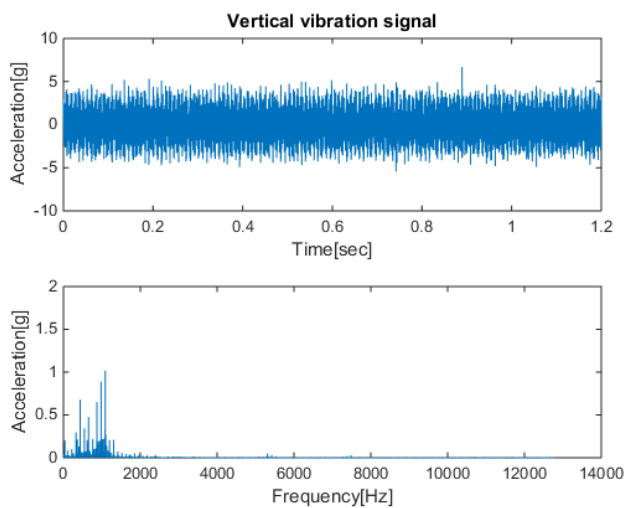
Fig. 5. Vertical vibration signal
