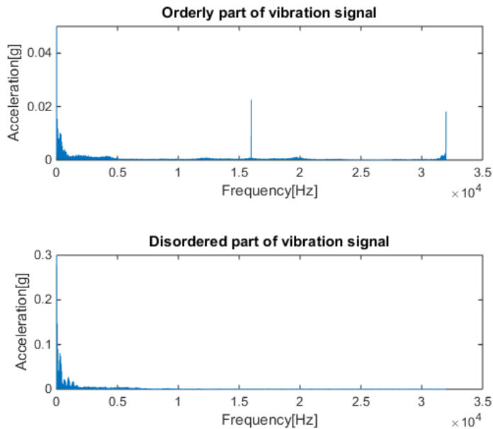
Fig. 13. Envelope spectrum of ordered and disordered parts
