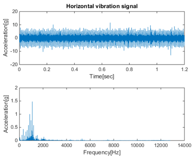
Fig. 4. Horizontal vibration signal
