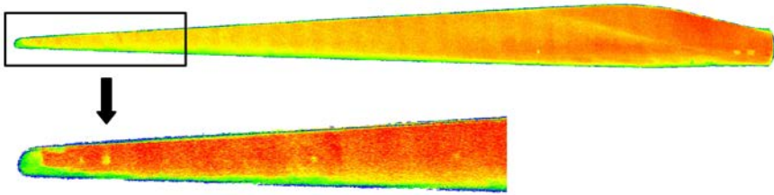
Fig. 10. Point cloud obtained for SS of blade B.
