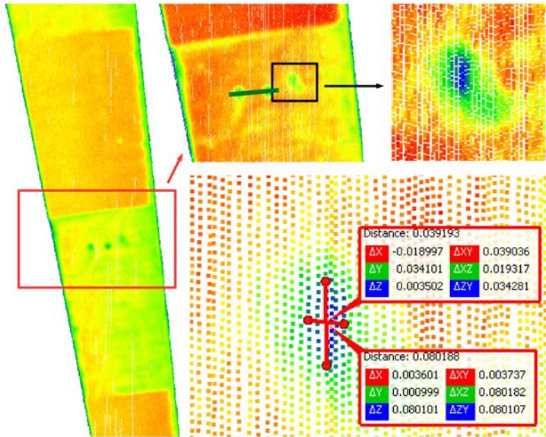
Fig. 12. Analysis result of small parts of the point cloud (a fragment from blade B').
