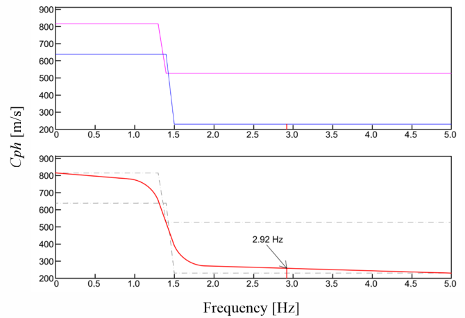
Fig. 7. Determined approximation of the dispersion curve for the adopted multi-layer soil
