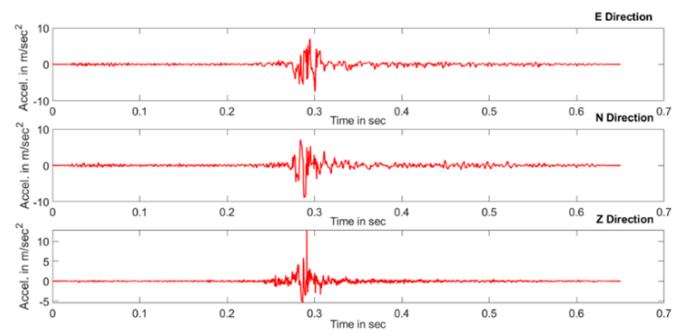
Fig. 8. Time course of ground accelerations in the N , E and Z directions for the tremor of 02-06-2023 near the city of Gaziantep, Turkey
