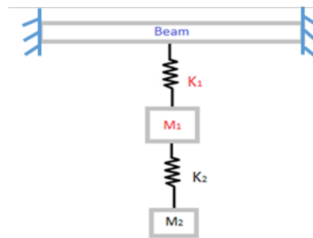
Fig. 3. Schematic representation of a beam structure attached with two DVA
