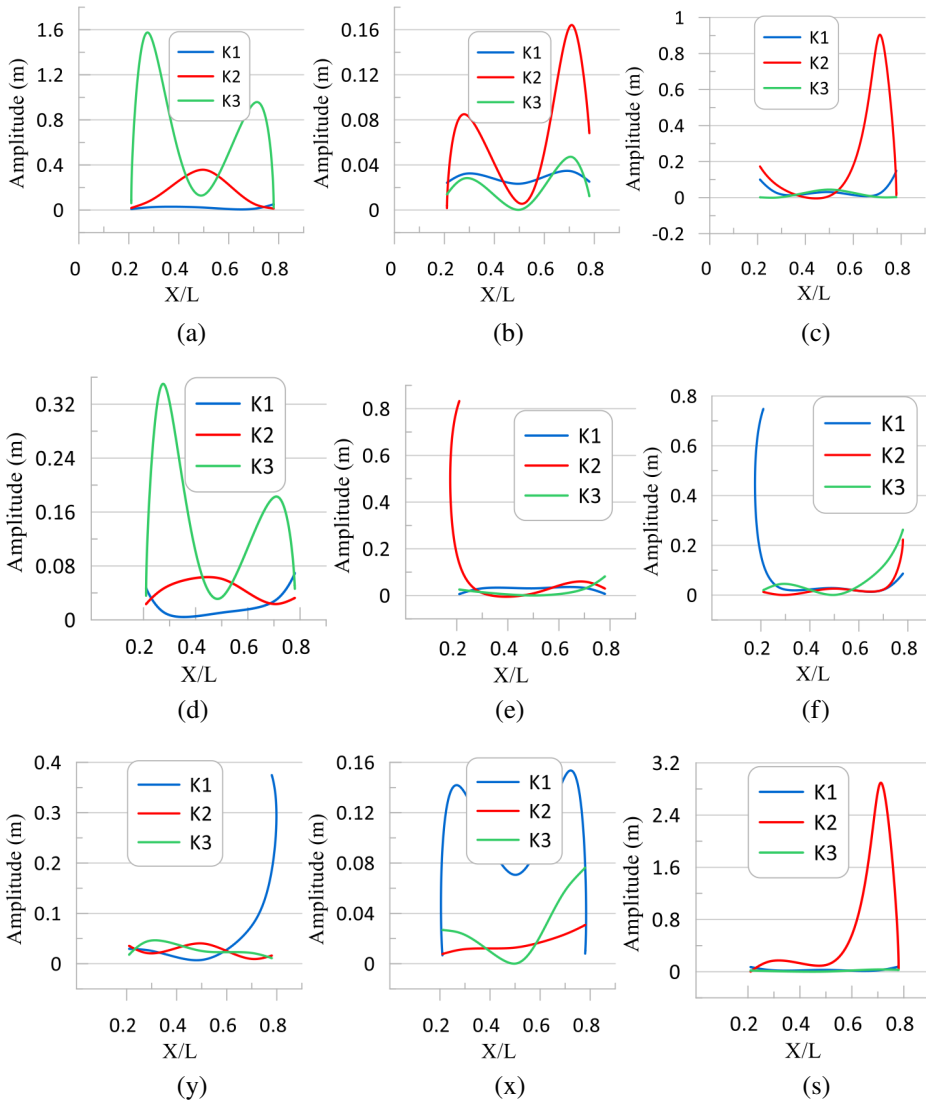
Fig. 16. The effect of DVA locations in harmonic response for three mode shapes; (a, b, and c) for M = 100 g; (d, e and f) for M = 200 g; (y, x, and s) for M = 300 g
