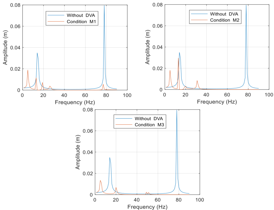
Fig. 13. Comparison of amplitudes between the cases without and with DVA for conditions M_1 , M_2 , and M_3
