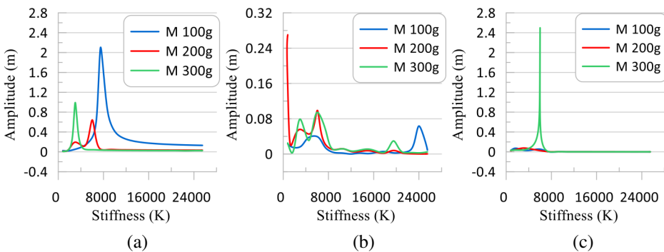
Fig. 15. The influence of stiffness on harmonic responsiveness for three mode shapes (a, b, and c)
