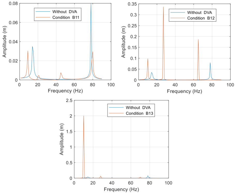
Fig. 5. Comparison of amplitudes between without and with DVA for conditions B 11 , B 12 and B 13
