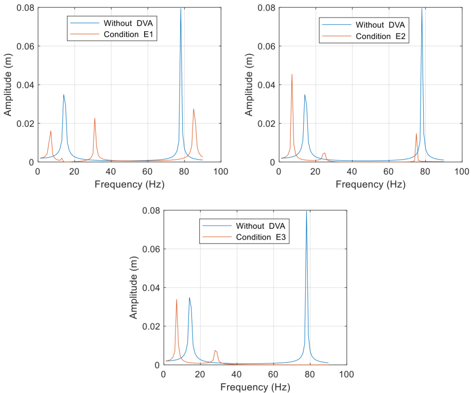
Fig. 10. Comparison of amplitudes between without and with DVA for conditions E_1 , E_2 and E_3
