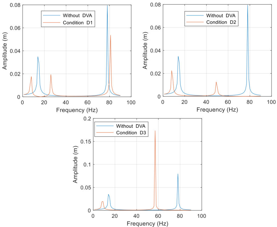
Fig. 9. Comparison of amplitudes between without and with DVA for conditions D_1 , D_2 and D_3
