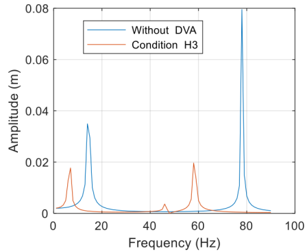
Fig. 12. Comparison of amplitudes between without and with DVA for conditions H_1 , H_2 and H_3
