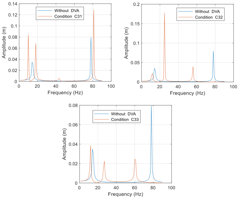
Fig. 8. Comparison of amplitudes between without and with DVA for conditions C_{31} , C_{32} and C_{33}
