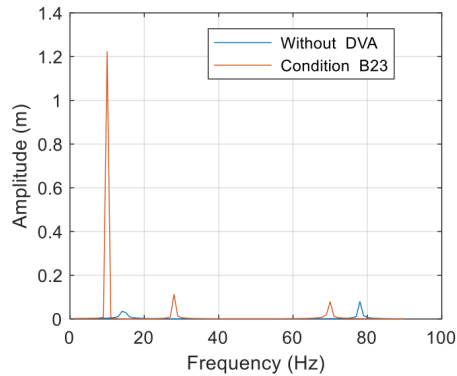
Fig. 6. Comparison of amplitudes between without and with DVA for conditions B 21 , B 22 and B 23
