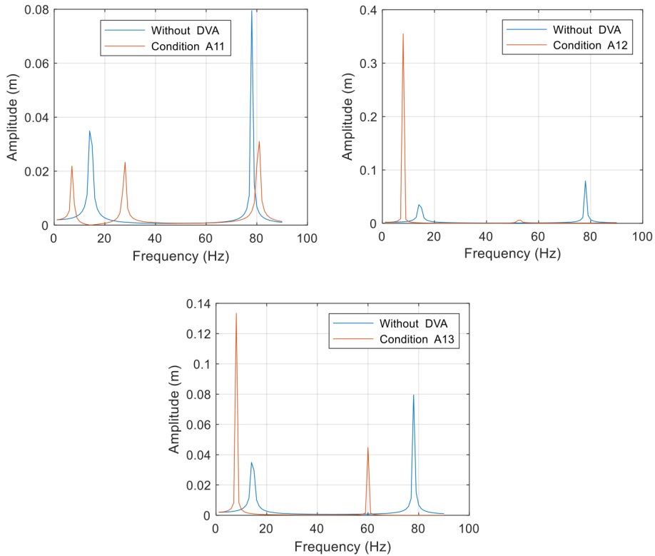
Fig. 4. Comparison of amplitudes between without and with DVA for conditions A_{11} , A_{12} and A_{13}
