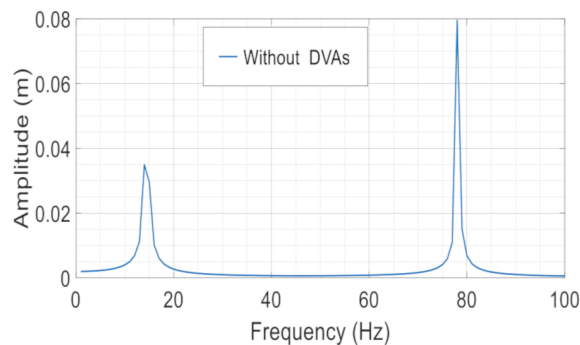
Fig. 2. Dynamic response without DVA
