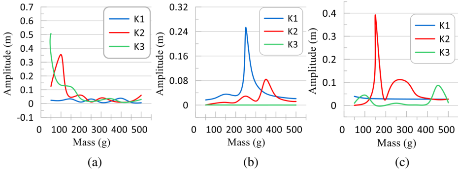
Fig. 14. The influence of mass on harmonic responsiveness for three mode shapes (a, b, and c)
