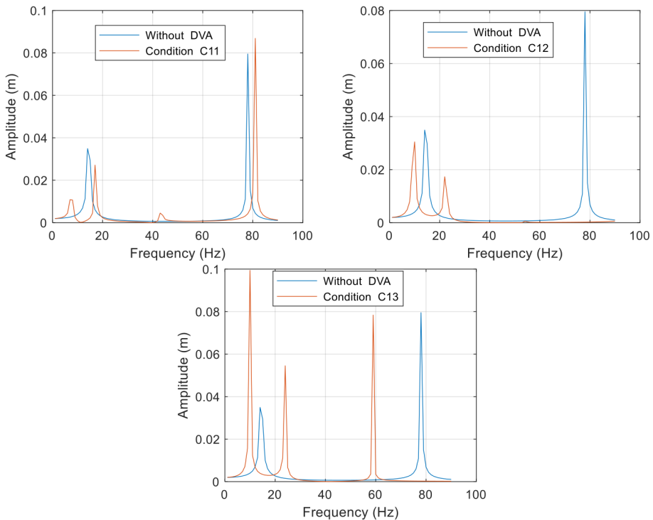
Fig. 7. Comparison of amplitudes between without and with DVA for conditions C 11 , C 12 and C 13
