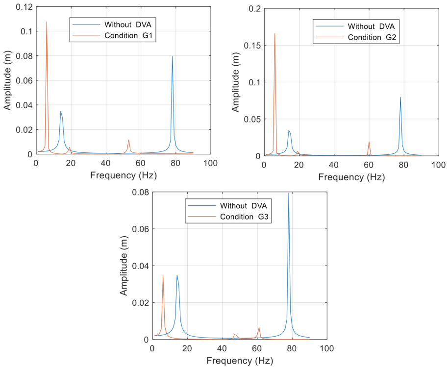
Fig. 11. Comparison of amplitudes between without and with DVA for conditions G_1 , G_2 and G_3
