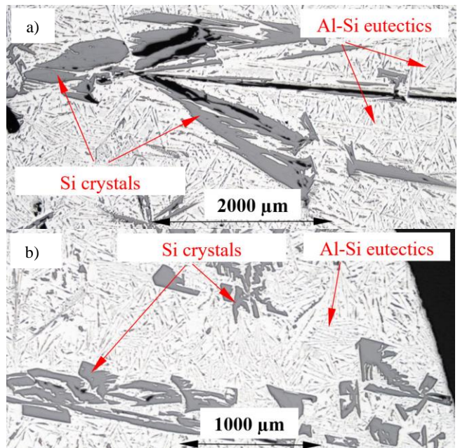
Fig. 6. Microstructures of the Si-first (AlSi14.734Mn0.567) alloy specimen solidified by flux: (a) 0 mT and (b) 11 mT of electromagnetic field. LOM, magnification 100×
