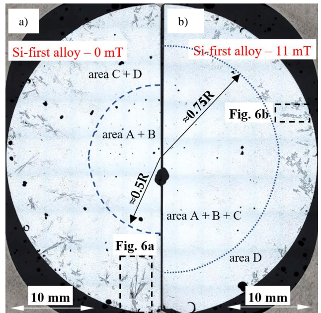
Fig. 5. Microstructures of: the Si-first (AlSi14.732Mn0.567) alloy specimen solidified by flux: (a) 0 mT and (b) 11 mT of electromagnetic field. LOM, magnification 25×
