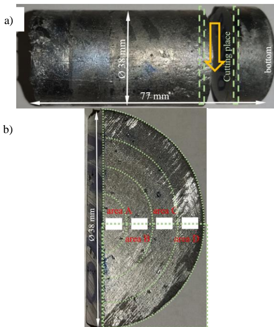
Fig. 2. Processed specimens: a) place for cutting the cross-section, b) areas A, B, C and D for parameters measurement. The dashed green line area used for general observation. The dotted green line show arch shaped area for the measurement of Si crystals, large Mn intermetallics and dendrite arm spacing (magnification 50\times ). The rectangle shaped white-filled areas were determined for e.g. eutectic spacing measurement (magnification 50\times and 200\times )
