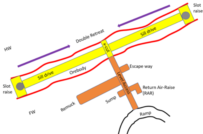
Fig. 6. Development of MSLC Mining Level
