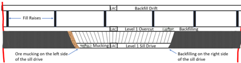
Fig. 8f. Concurrent Mining and Backfilling Activities
