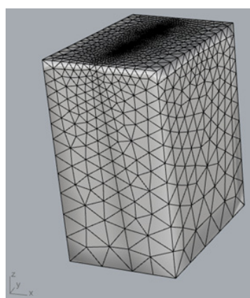
Fig. 18. Isometric view of the Rhino model
