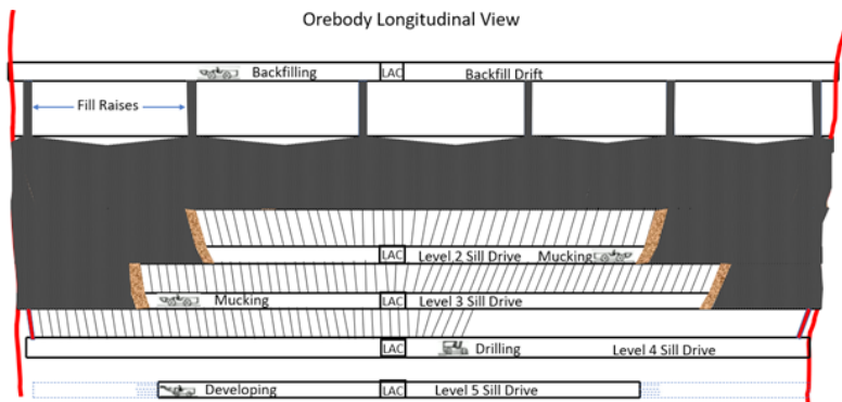
Fig. 11. Mining Level 1 Completed
