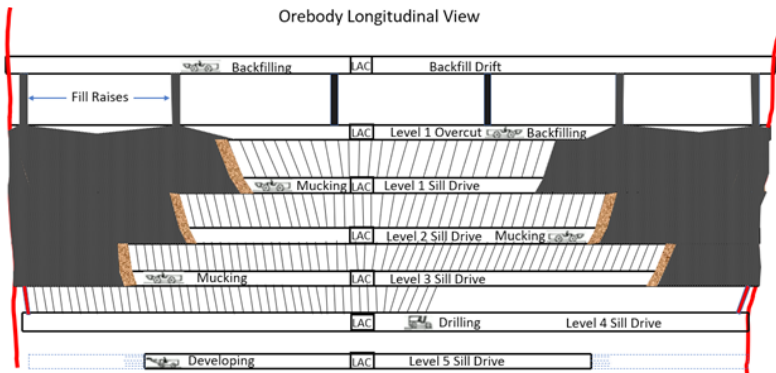
Fig. 10. Multi-level Mining
