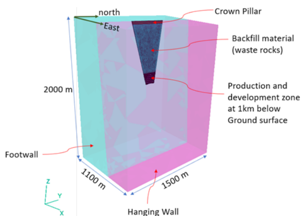
Fig. 19. Isometric view of FLAC3D mine-wide model
